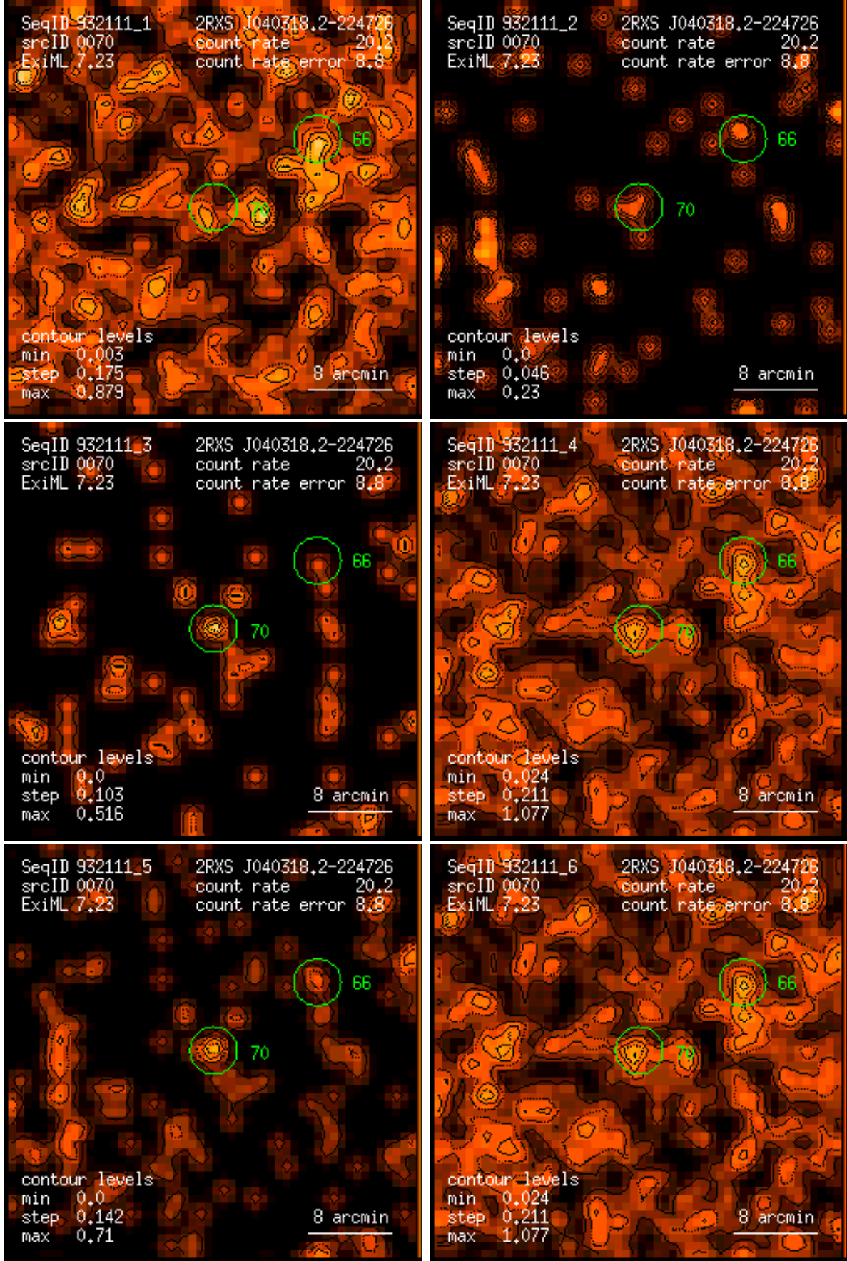
Figure 70: RASS 932111: detection 0070: band rate images, Gaussian filter: (1) PSPC channels 11 – 41, (2) 52 – 90, (3) 91 – 201, (4) 11 – 235, (5) 52 – 201, (6) 11 – 201. Broad band rates in counts/ks. Band rate contour levels in counts/ks/arcmin 2 .
