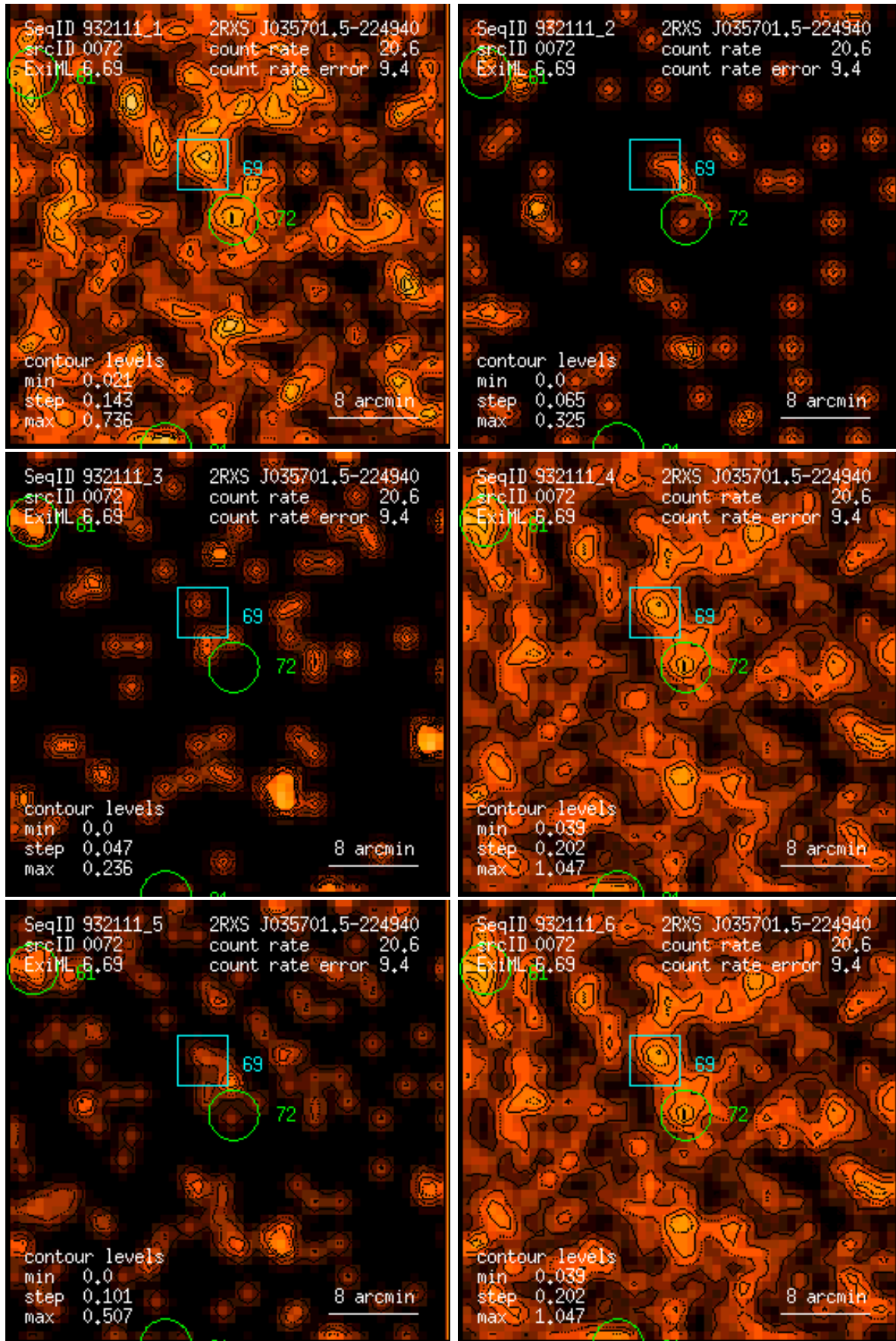
Figure 72: RASS 932111: detection 0072: band rate images, Gaussian filter: (1) PSPC channels 11 – 41, (2) 52 – 90, (3) 91 – 201, (4) 11 – 235, (5) 52 – 201, (6) 11 – 201. Broad band rates in counts/ks. Band rate contour levels in counts/ks/arcmin 2 .
