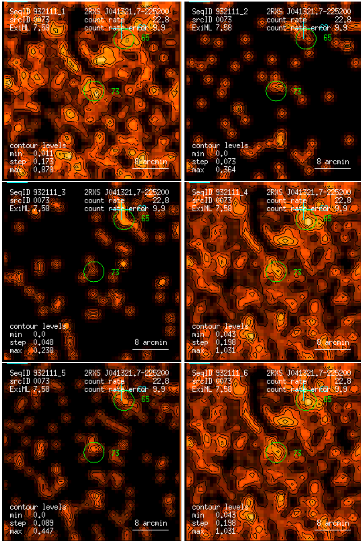
Figure 73: RASS 932111: detection 0073: band rate images, Gaussian filter: (1) PSPC channels 11 – 41, (2) 52 – 90, (3) 91 – 201, (4) 11 – 235, (5) 52 – 201, (6) 11 – 201. Broad band rates in counts/ks. Band rate contour levels in counts/ks/arcmin 2 .
