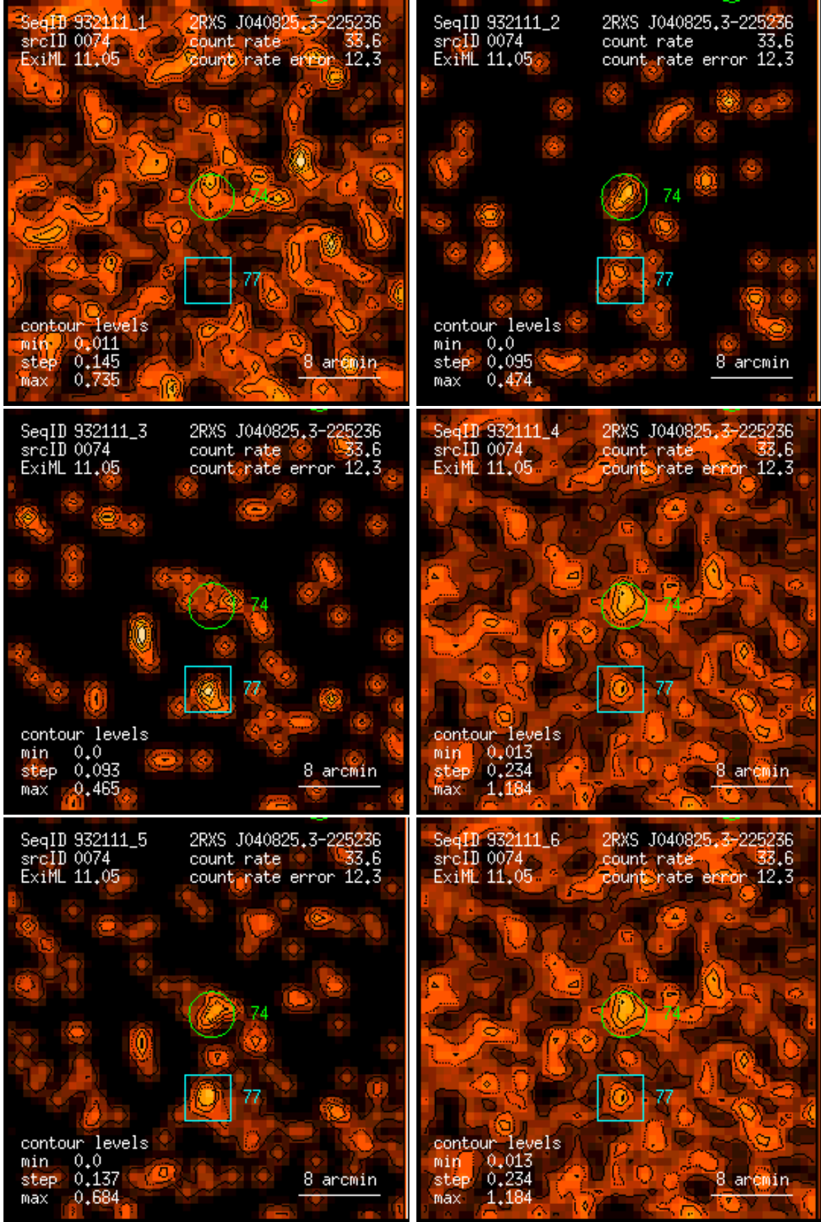
Figure 74: RASS 932111: detection 0074: band rate images, Gaussian filter: (1) PSPC channels 11 – 41, (2) 52 – 90, (3) 91 – 201, (4) 11 – 235, (5) 52 – 201, (6) 11 – 201. Broad band rates in counts/ks. Band rate contour levels in counts/ks/arcmin 2 .
