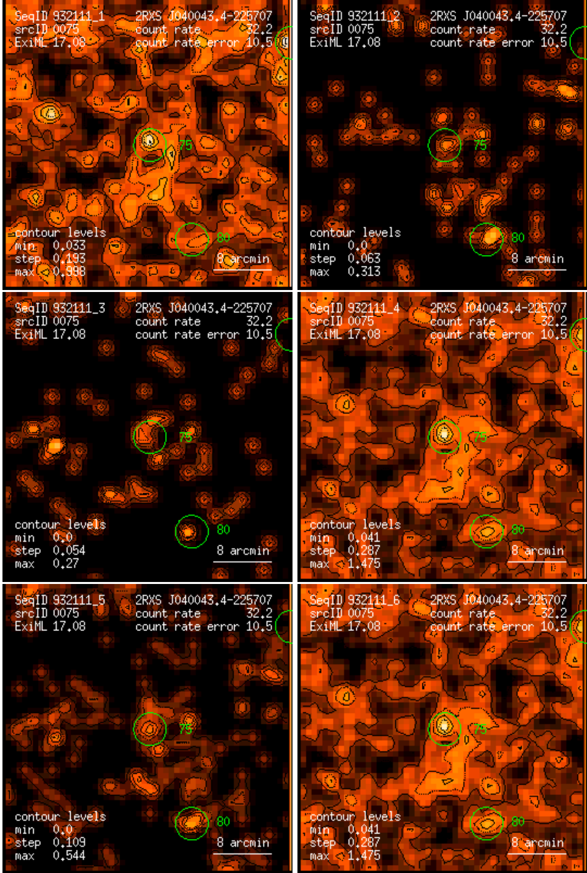
Figure 75: RASS 932111: detection 0075: band rate images, Gaussian filter: (1) PSPC channels 11 – 41, (2) 52 – 90, (3) 91 – 201, (4) 11 – 235, (5) 52 – 201, (6) 11 – 201. Broad band rates in counts/ks. Band rate contour levels in counts/ks/arcmin 2 .
