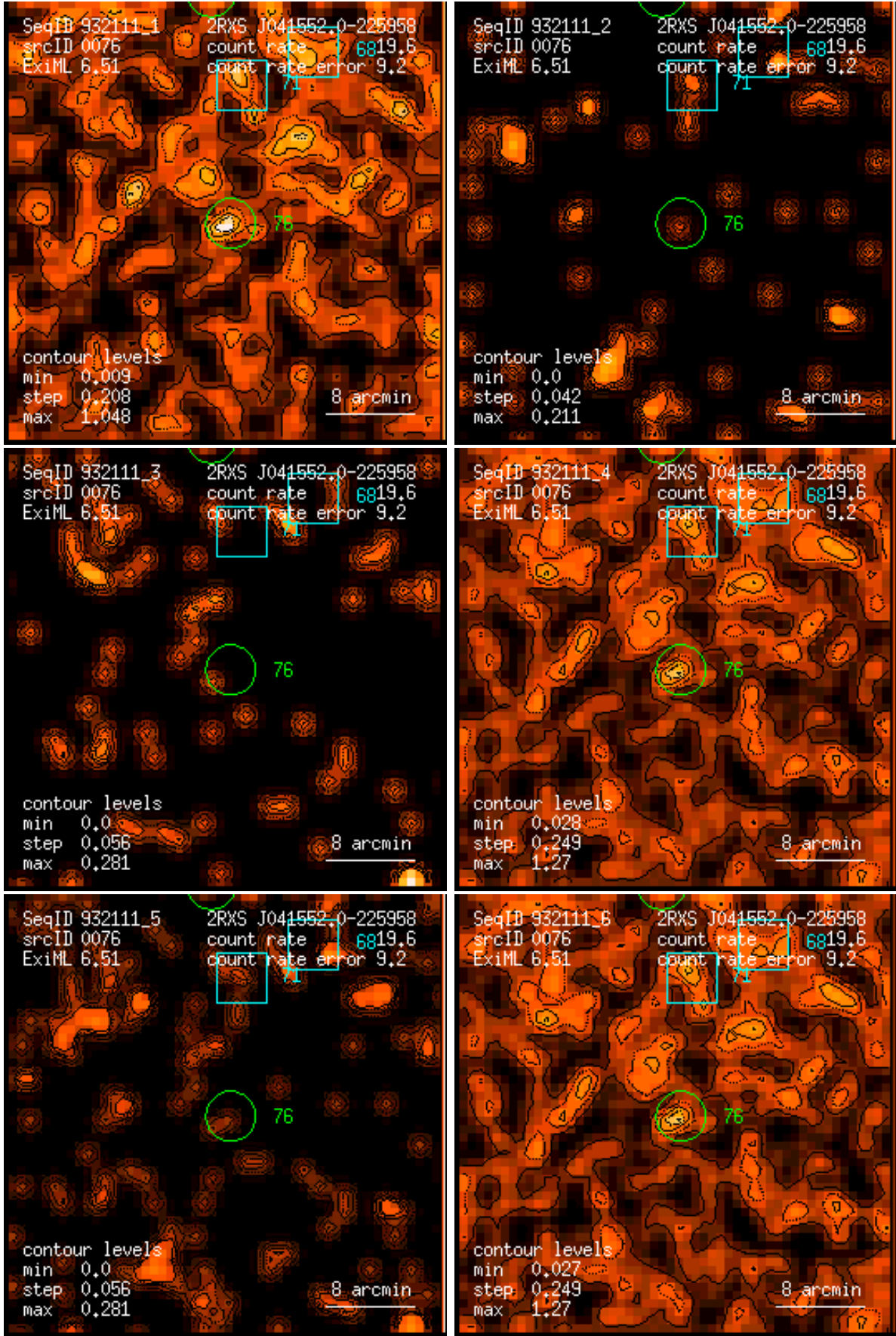
Figure 76: RASS 932111: detection 0076: band rate images, Gaussian filter: (1) PSPC channels 11 – 41, (2) 52 – 90, (3) 91 – 201, (4) 11 – 235, (5) 52 – 201, (6) 11 – 201. Broad band rates in counts/ks. Band rate contour levels in counts/ks/arcmin 2 .
