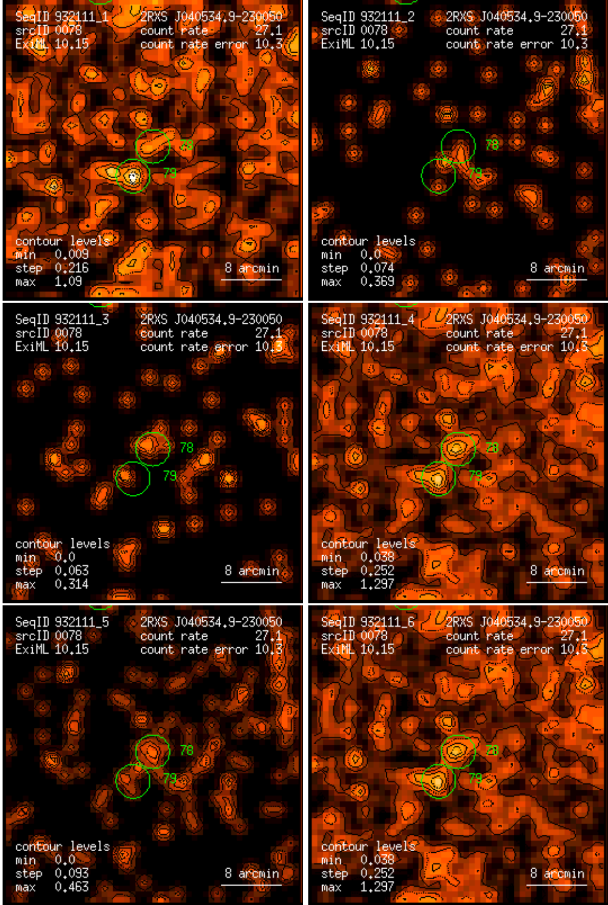
Figure 78: RASS 932111: detection 0078: band rate images, Gaussian filter: (1) PSPC channels 11 – 41, (2) 52 – 90, (3) 91 – 201, (4) 11 – 235, (5) 52 – 201, (6) 11 – 201. Broad band rates in counts/ks. Band rate contour levels in counts/ks/arcmin 2 .
