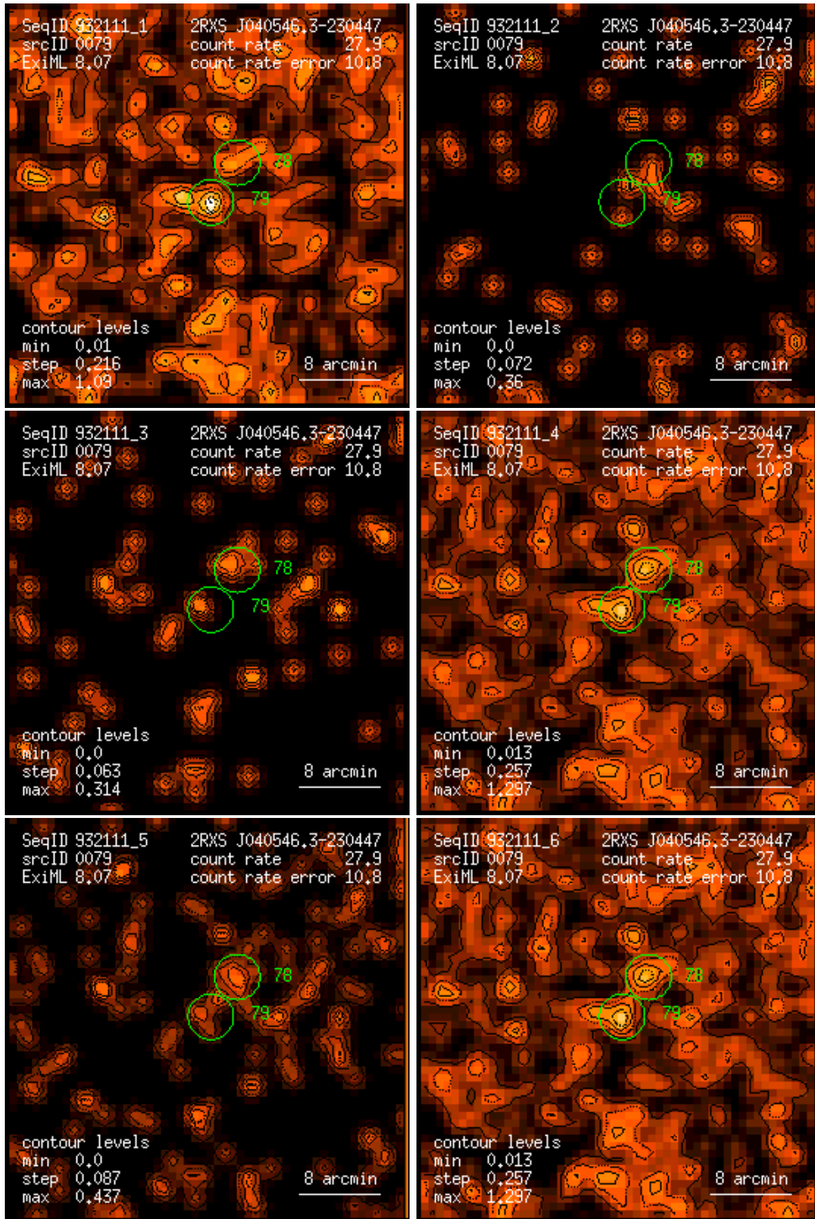
Figure 79: RASS 932111: detection 0079: band rate images, Gaussian filter: (1) PSPC channels 11 – 41, (2) 52 – 90, (3) 91 – 201, (4) 11 – 235, (5) 52 – 201, (6) 11 – 201. Broad band rates in counts/ks. Band rate contour levels in counts/ks/arcmin 2 .
