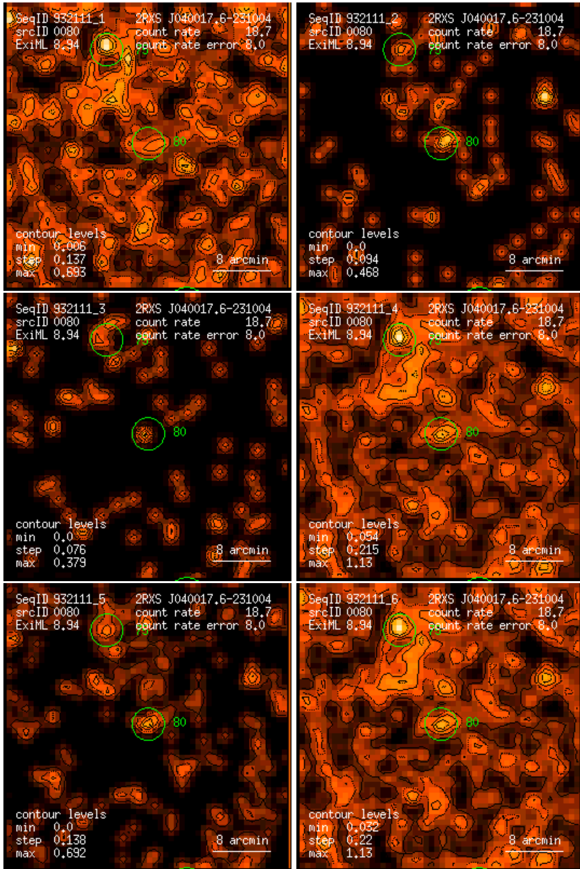
Figure 80: RASS 932111: detection 0080: band rate images, Gaussian filter: (1) PSPC channels 11 – 41, (2) 52 – 90, (3) 91 – 201, (4) 11 – 235, (5) 52 – 201, (6) 11 – 201. Broad band rates in counts/ks. Band rate contour levels in counts/ks/arcmin 2 .
