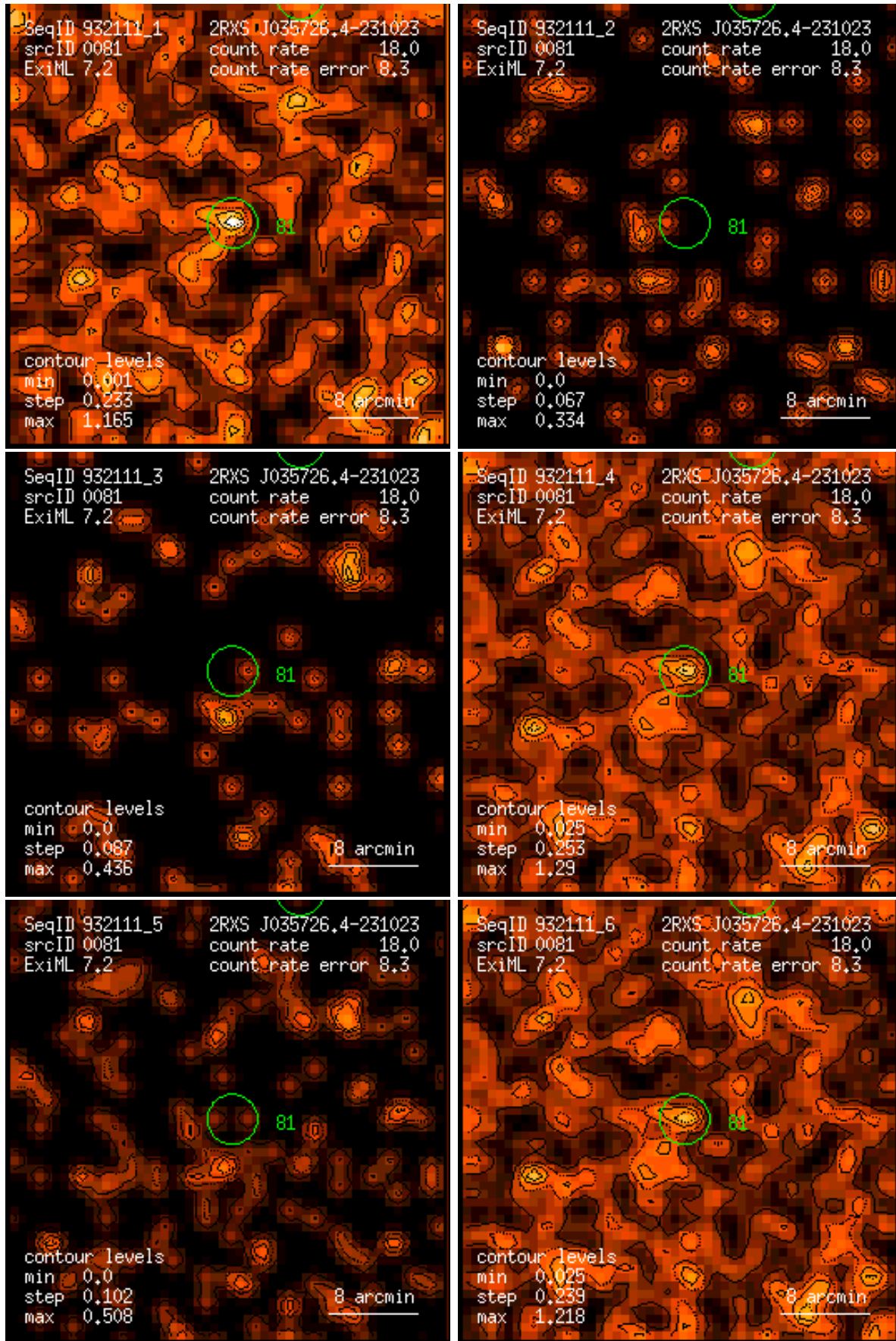
Figure 81: RASS 932111: detection 0081: band rate images, Gaussian filter: (1) PSPC channels 11 – 41, (2) 52 – 90, (3) 91 – 201, (4) 11 – 235, (5) 52 – 201, (6) 11 – 201. Broad band rates in counts/ks. Band rate contour levels in counts/ks/arcmin 2 .
