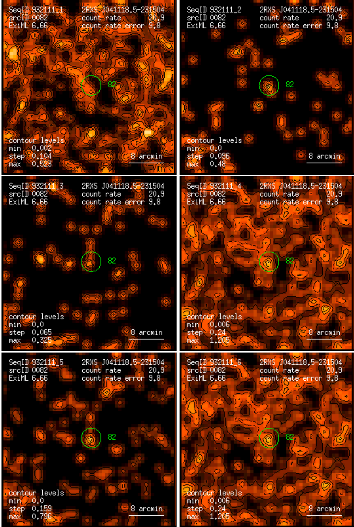
Figure 82: RASS 932111: detection 0082: band rate images, Gaussian filter: (1) PSPC channels 11 – 41, (2) 52 – 90, (3) 91 – 201, (4) 11 – 235, (5) 52 – 201, (6) 11 – 201. Broad band rates in counts/ks. Band rate contour levels in counts/ks/arcmin 2 .
