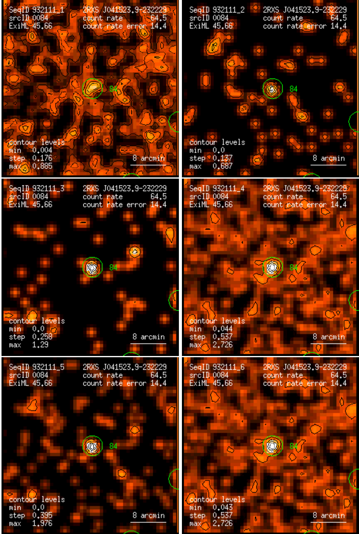
Figure 84: RASS 932111: detection 0084: band rate images, Gaussian filter: (1) PSPC channels 11 – 41, (2) 52 – 90, (3) 91 – 201, (4) 11 – 235, (5) 52 – 201, (6) 11 – 201. Broad band rates in counts/ks. Band rate contour levels in counts/ks/arcmin 2 .
