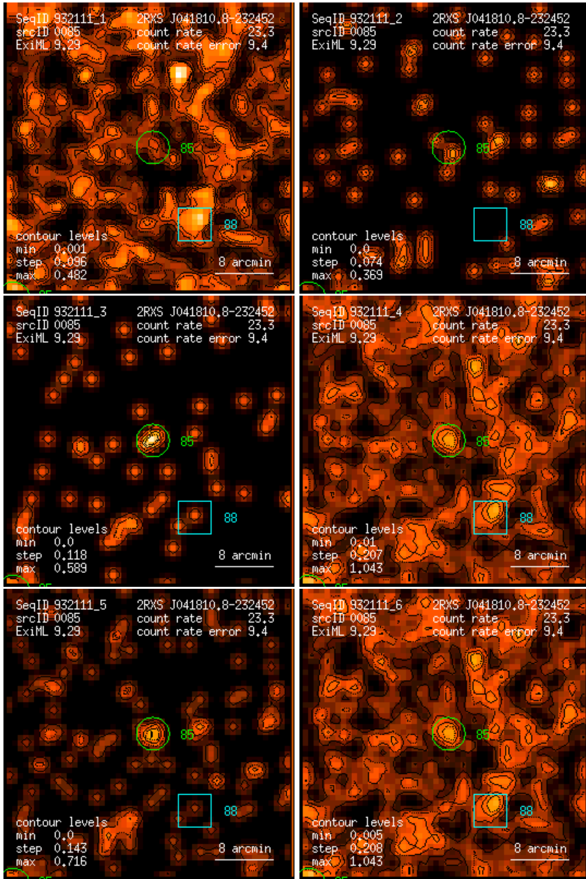
Figure 85: RASS 932111: detection 0085: band rate images, Gaussian filter: (1) PSPC channels 11 – 41, (2) 52 – 90, (3) 91 – 201, (4) 11 – 235, (5) 52 – 201, (6) 11 – 201. Broad band rates in counts/ks. Band rate contour levels in counts/ks/arcmin 2 .
