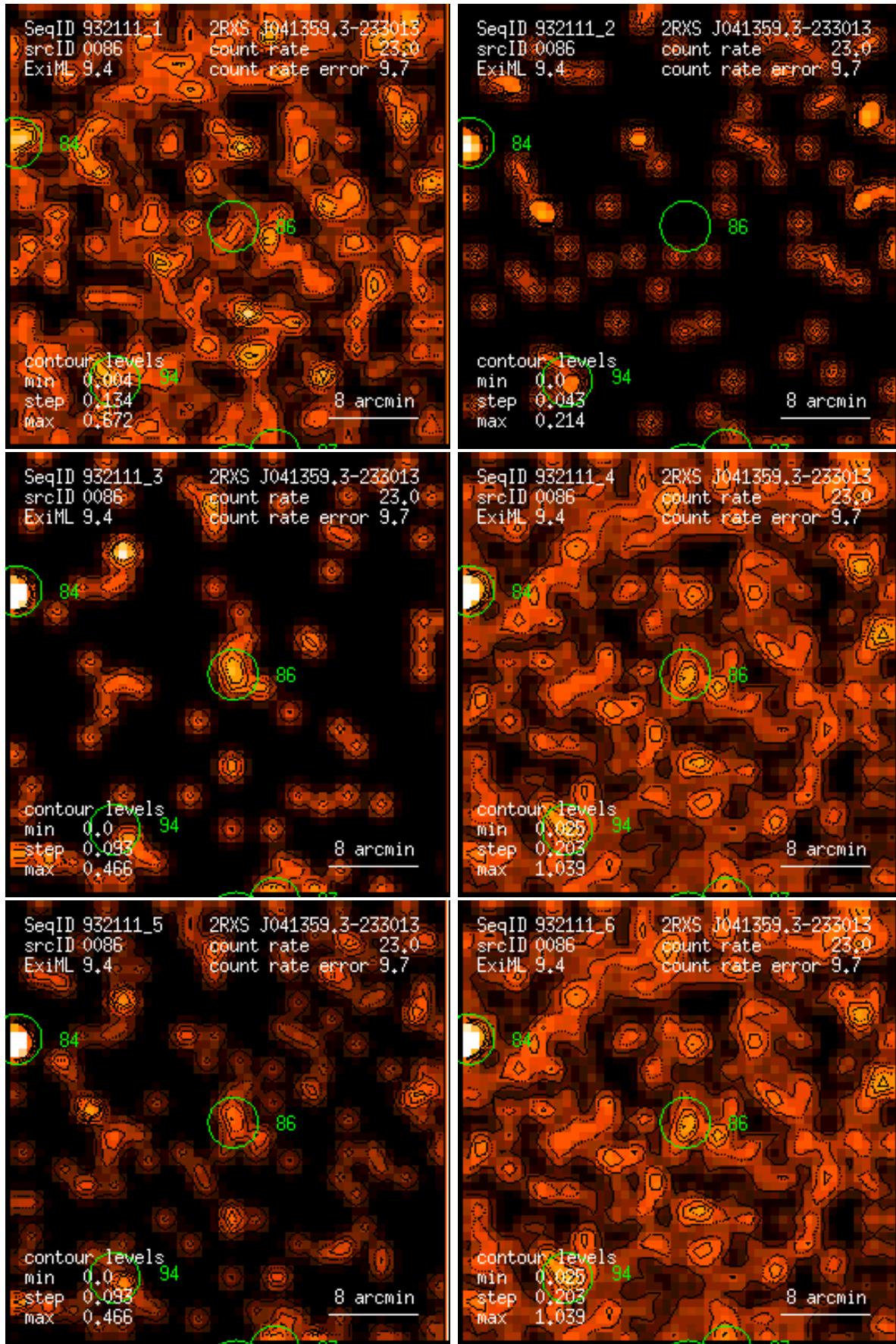
Figure 86: RASS 932111: detection 0086: band rate images, Gaussian filter: (1) PSPC channels 11 – 41, (2) 52 – 90, (3) 91 – 201, (4) 11 – 235, (5) 52 – 201, (6) 11 – 201. Broad band rates in counts/ks. Band rate contour levels in counts/ks/arcmin 2 .
