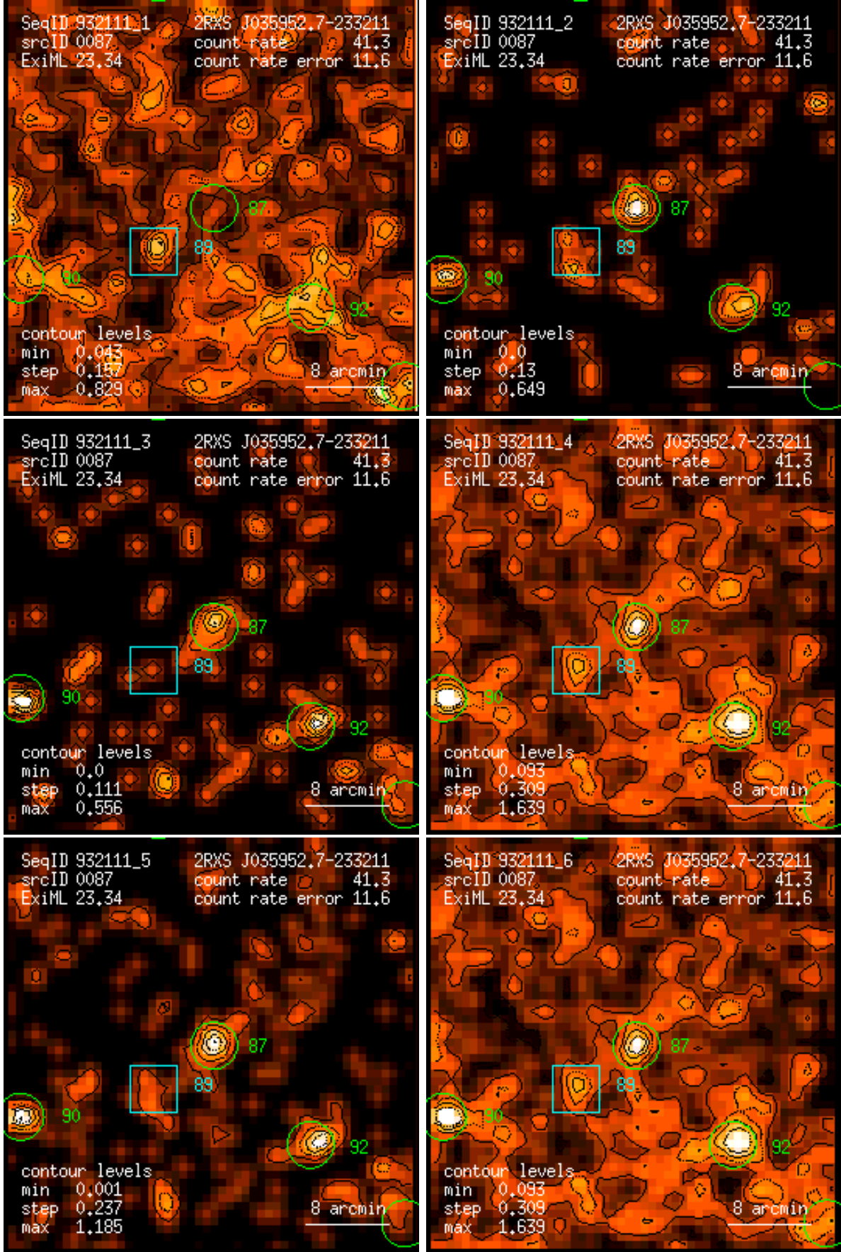
Figure 87: RASS 932111: detection 0087: band rate images, Gaussian filter: (1) PSPC channels 11 – 41, (2) 52 – 90, (3) 91 – 201, (4) 11 – 235, (5) 52 – 201, (6) 11 – 201. Broad band rates in counts/ks. Band rate contour levels in counts/ks/arcmin 2 .
