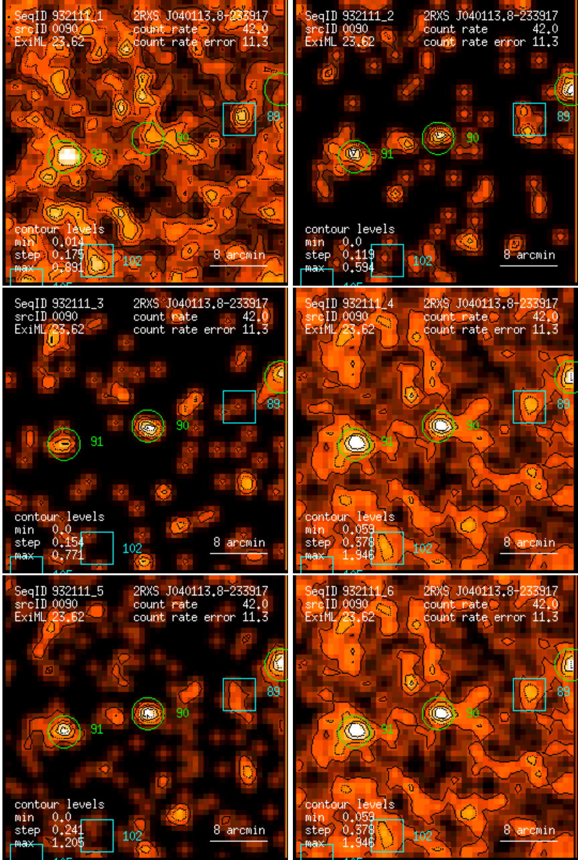
Figure 90: RASS 932111: detection 0090: band rate images, Gaussian filter: (1) PSPC channels 11 – 41, (2) 52 – 90, (3) 91 – 201, (4) 11 – 235, (5) 52 – 201, (6) 11 – 201. Broad band rates in counts/ks. Band rate contour levels in counts/ks/arcmin 2 .
