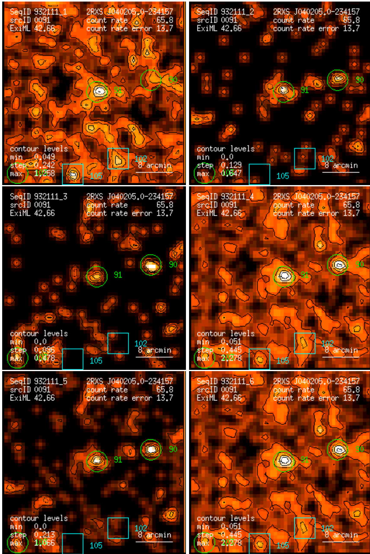
Figure 91: RASS 932111: detection 0091: band rate images, Gaussian filter: (1) PSPC channels 11 – 41, (2) 52 – 90, (3) 91 – 201, (4) 11 – 235, (5) 52 – 201, (6) 11 – 201. Broad band rates in counts/ks. Band rate contour levels in counts/ks/arcmin 2 .
