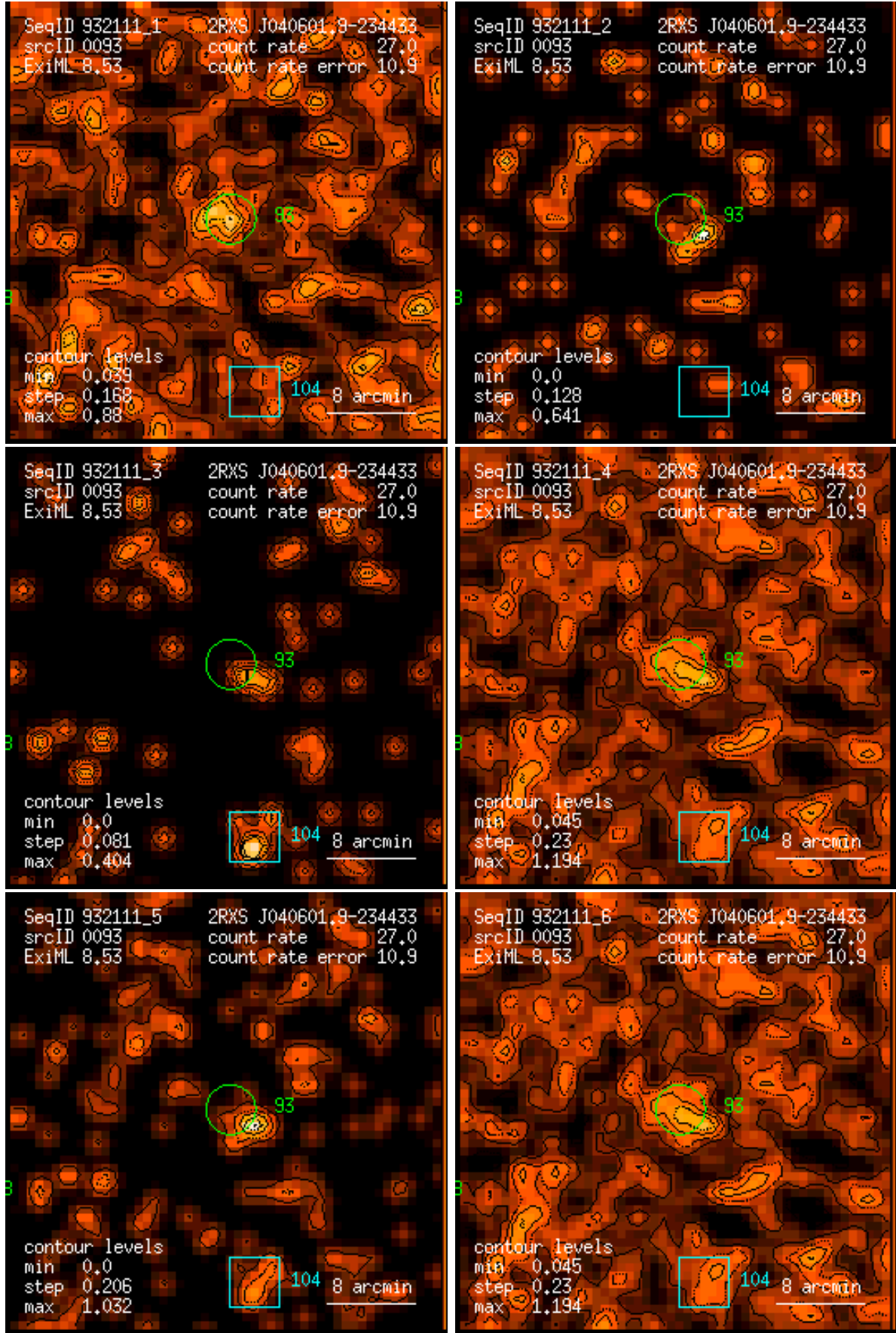
Figure 93: RASS 932111: detection 0093: band rate images, Gaussian filter: (1) PSPC channels 11 – 41, (2) 52 – 90, (3) 91 – 201, (4) 11 – 235, (5) 52 – 201, (6) 11 – 201. Broad band rates in counts/ks. Band rate contour levels in counts/ks/arcmin 2 .
