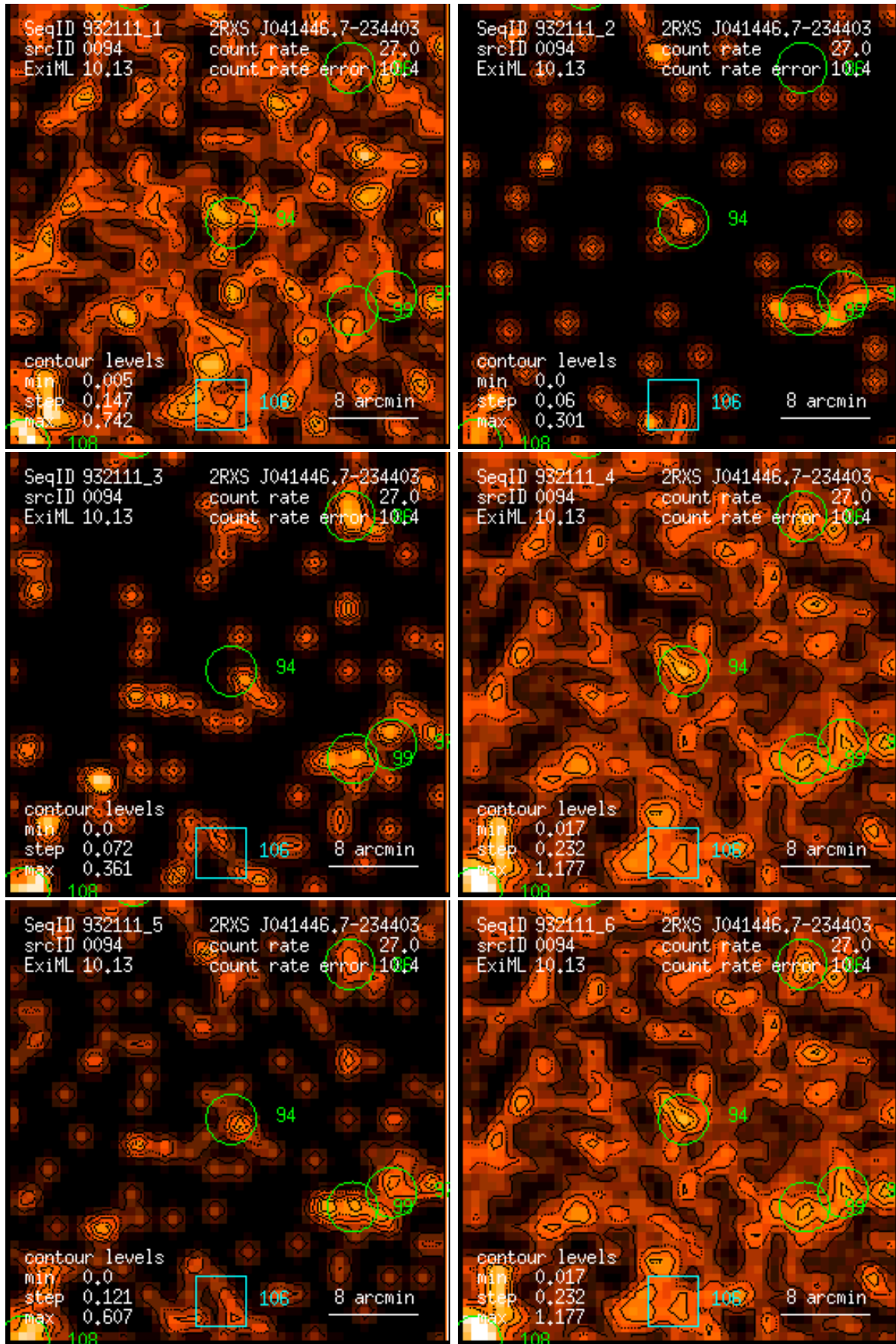
Figure 94: RASS 932111: detection 0094: band rate images, Gaussian filter: (1) PSPC channels 11 – 41, (2) 52 – 90, (3) 91 – 201, (4) 11 – 235, (5) 52 – 201, (6) 11 – 201. Broad band rates in counts/ks. Band rate contour levels in counts/ks/arcmin 2 .
