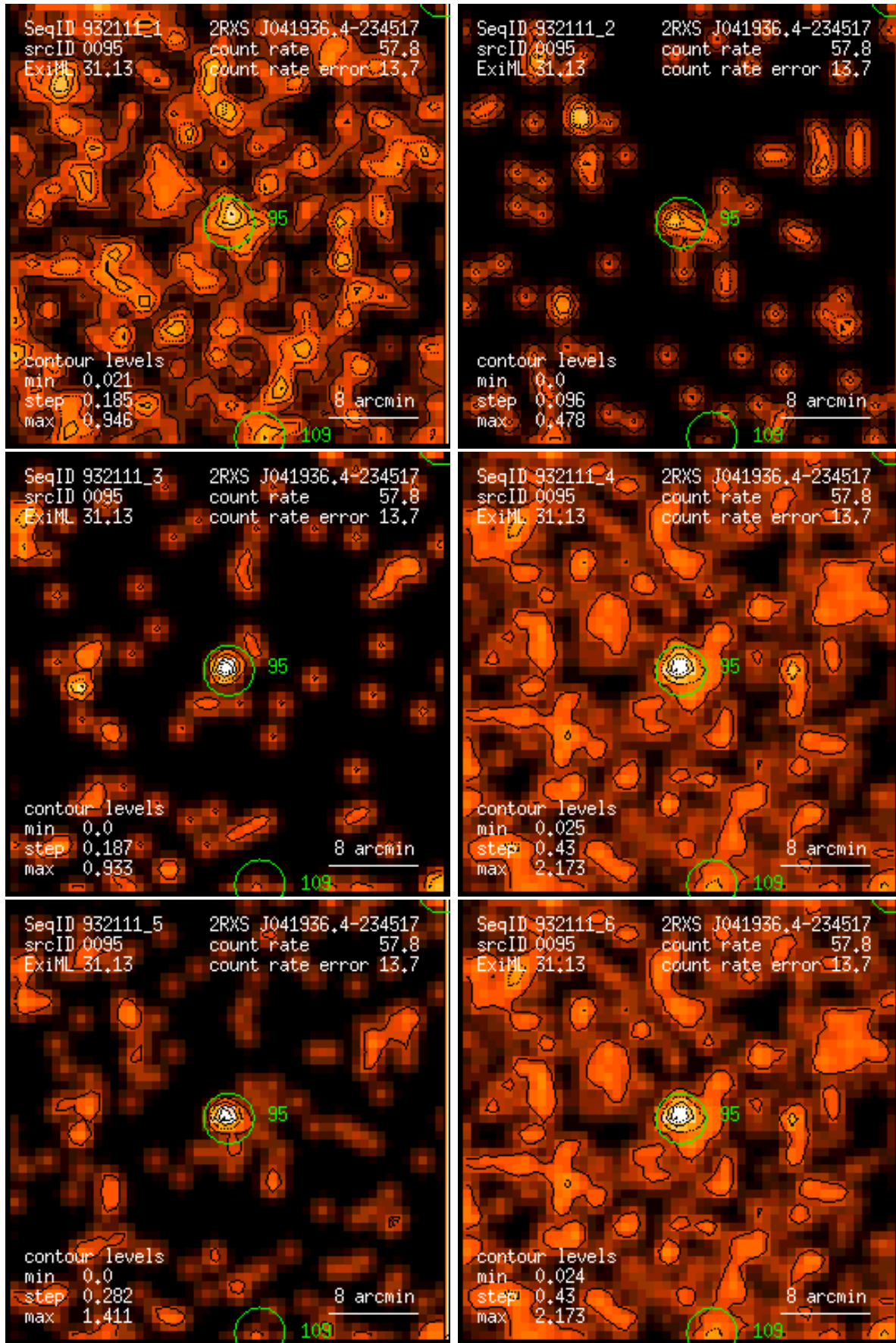
Figure 95: RASS 932111: detection 0095: band rate images, Gaussian filter: (1) PSPC channels 11 – 41, (2) 52 – 90, (3) 91 – 201, (4) 11 – 235, (5) 52 – 201, (6) 11 – 201. Broad band rates in counts/ks. Band rate contour levels in counts/ks/arcmin 2 .
