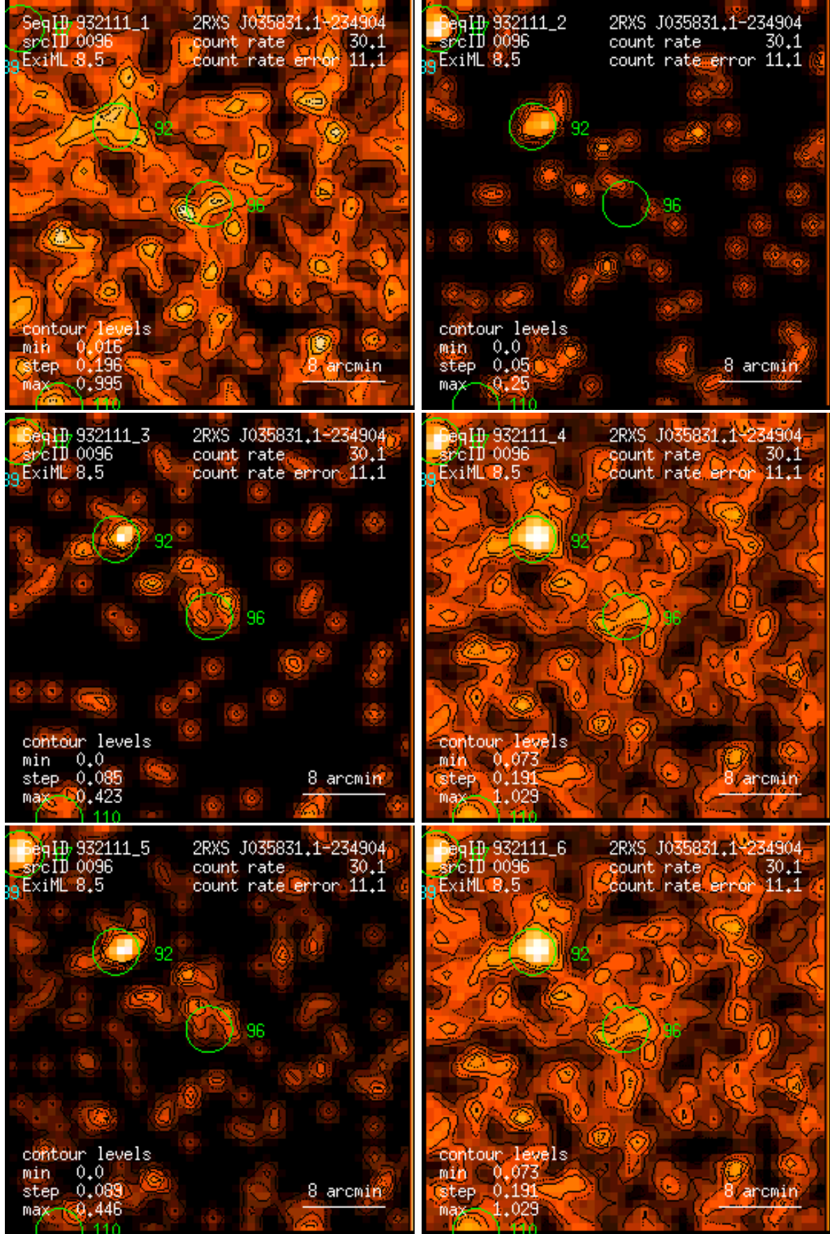
Figure 96: RASS 932111: detection 0096: band rate images, Gaussian filter: (1) PSPC channels 11 – 41, (2) 52 – 90, (3) 91 – 201, (4) 11 – 235, (5) 52 – 201, (6) 11 – 201. Broad band rates in counts/ks. Band rate contour levels in counts/ks/arcmin 2 .
