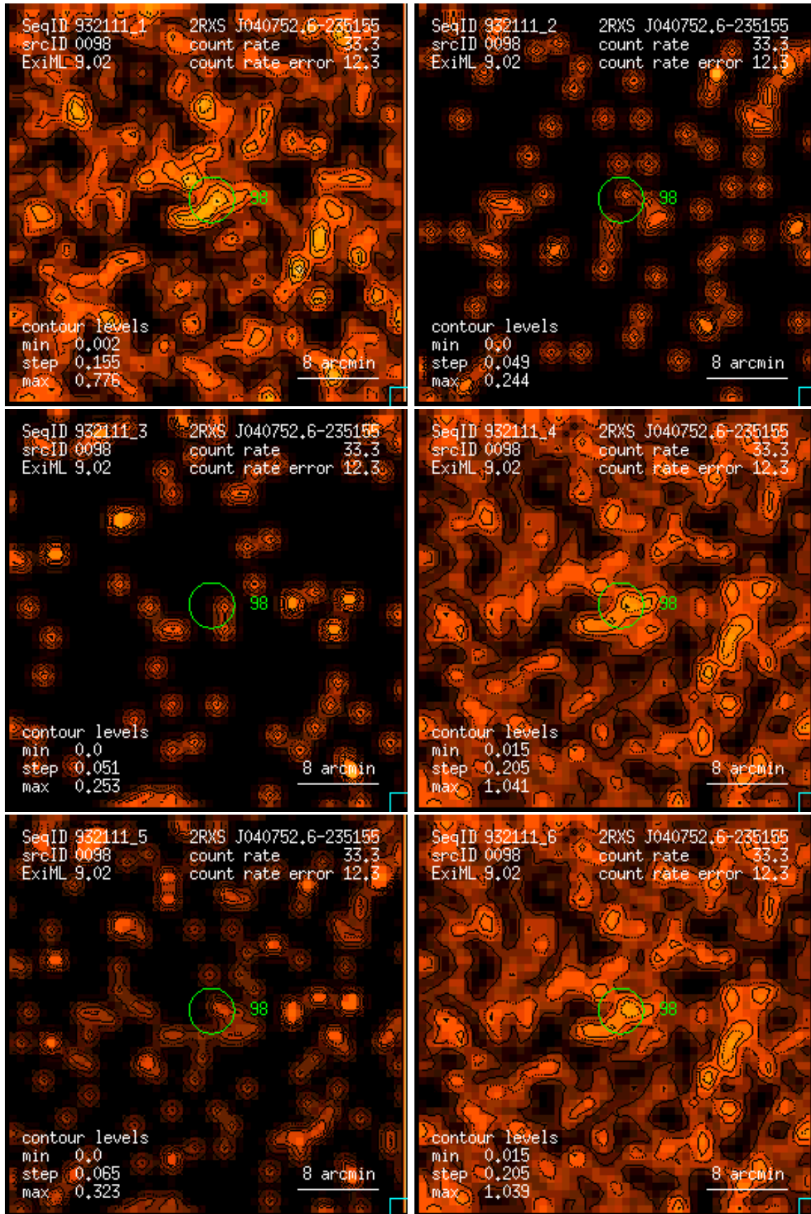
Figure 98: RASS 932111: detection 0098: band rate images, Gaussian filter: (1) PSPC channels 11 – 41, (2) 52 – 90, (3) 91 – 201, (4) 11 – 235, (5) 52 – 201, (6) 11 – 201. Broad band rates in counts/ks. Band rate contour levels in counts/ks/arcmin 2 .
