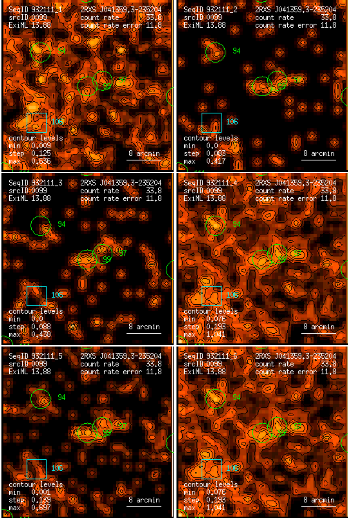
Figure 99: RASS 932111: detection 0099: band rate images, Gaussian filter: (1) PSPC channels 11 – 41, (2) 52 – 90, (3) 91 – 201, (4) 11 – 235, (5) 52 – 201, (6) 11 – 201. Broad band rates in counts/ks. Band rate contour levels in counts/ks/arcmin 2 .
