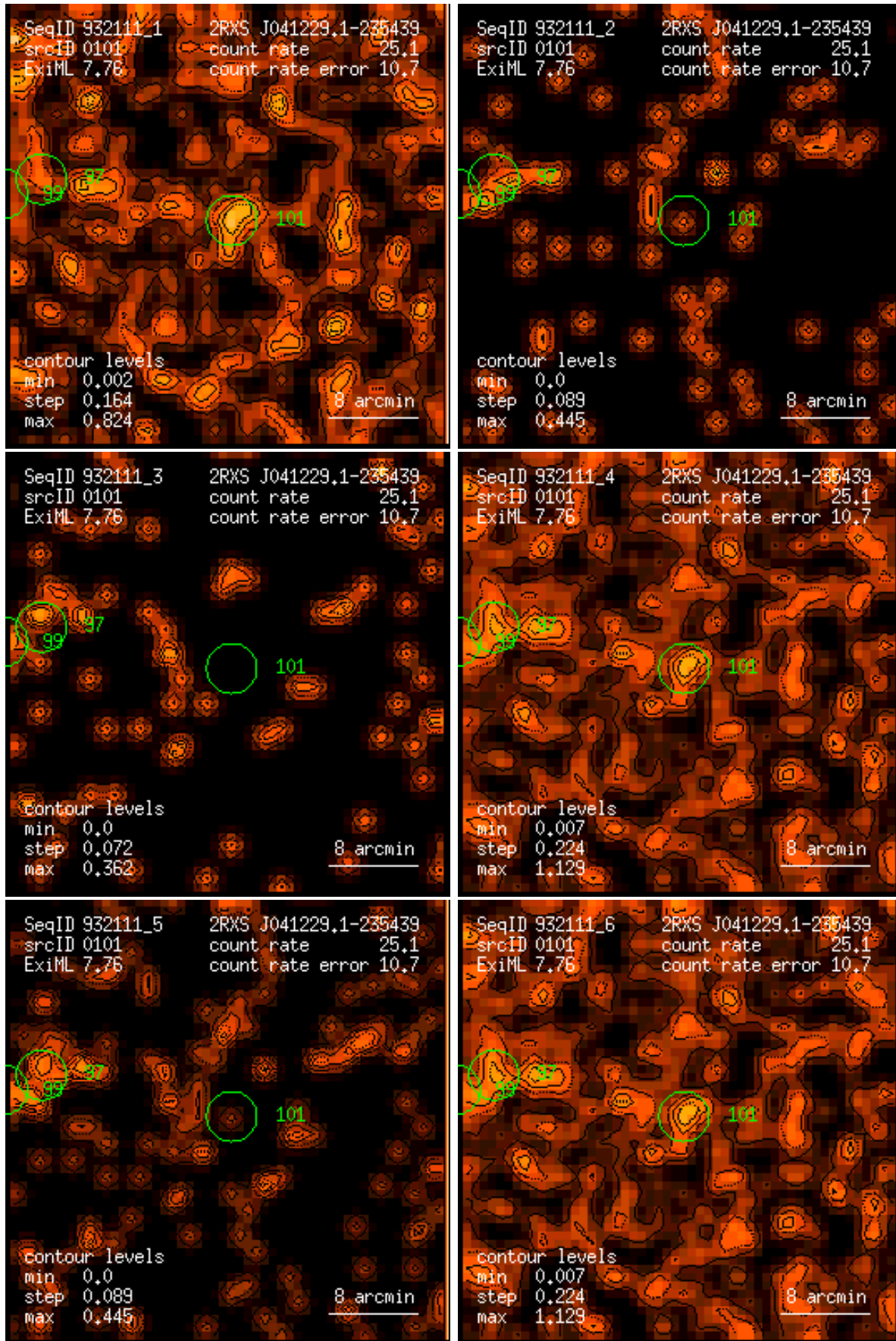
Figure 101: RASS 932111: detection 0101: band rate images, Gaussian filter: (1) PSPC channels 11 – 41, (2) 52 – 90, (3) 91 – 201, (4) 11 – 235, (5) 52 – 201, (6) 11 – 201. Broad band rates in counts/ks. Band rate contour levels in counts/ks/arcmin 2 .
