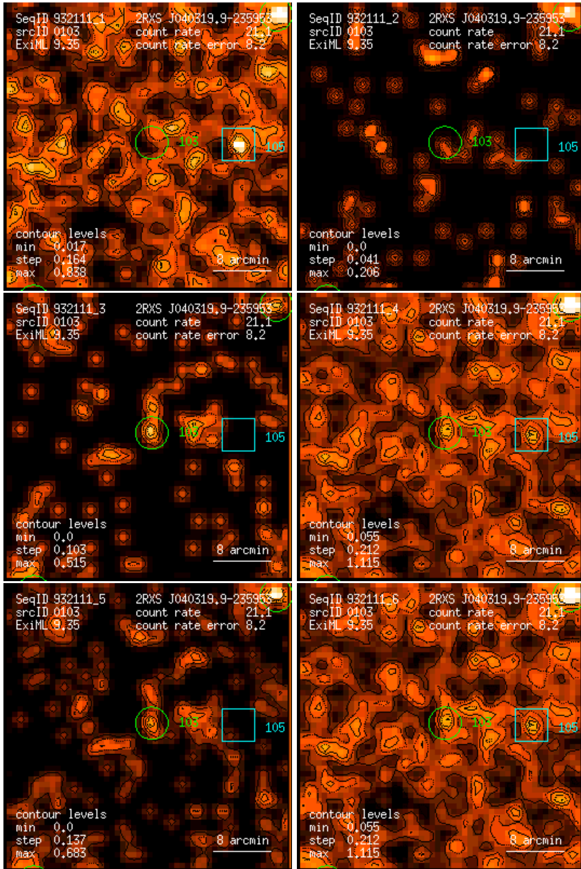
Figure 103: RASS 932111: detection 0103: band rate images, Gaussian filter: (1) PSPC channels 11 – 41, (2) 52 – 90, (3) 91 – 201, (4) 11 – 235, (5) 52 – 201, (6) 11 – 201. Broad band rates in counts/ks. Band rate contour levels in counts/ks/arcmin 2 .
