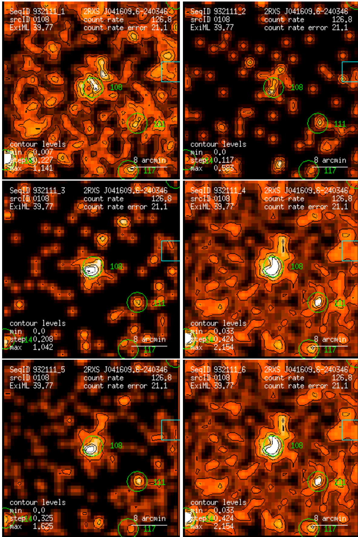
Figure 108: RASS 932111: detection 0108: band rate images, Gaussian filter: (1) PSPC channels 11 – 41, (2) 52 – 90, (3) 91 – 201, (4) 11 – 235, (5) 52 – 201, (6) 11 – 201. Broad band rates in counts/ks. Band rate contour levels in counts/ks/arcmin 2 .
