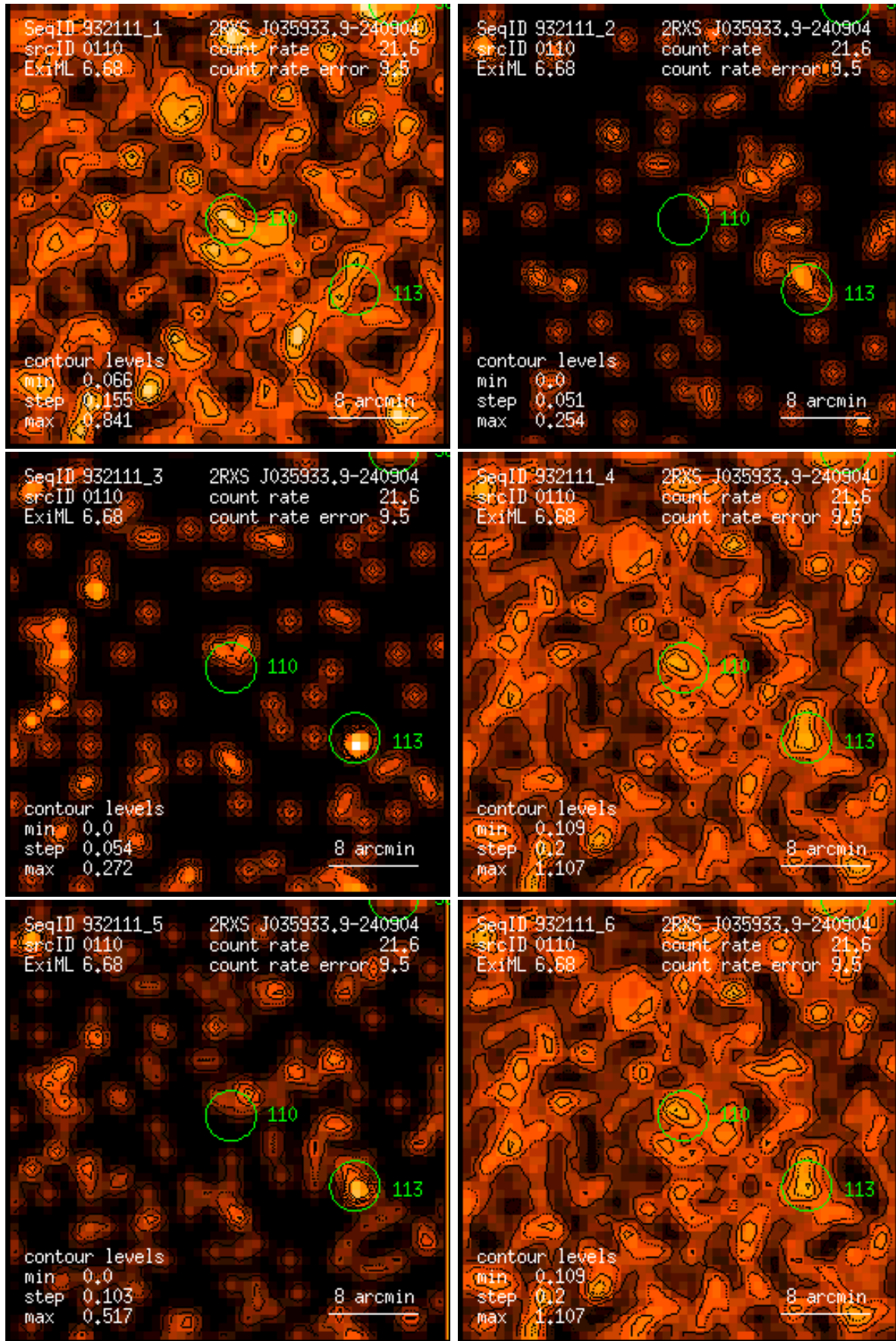
Figure 110: RASS 932111: detection 0110: band rate images, Gaussian filter: (1) PSPC channels 11 – 41, (2) 52 – 90, (3) 91 – 201, (4) 11 – 235, (5) 52 – 201, (6) 11 – 201. Broad band rates in counts/ks. Band rate contour levels in counts/ks/arcmin 2 .
