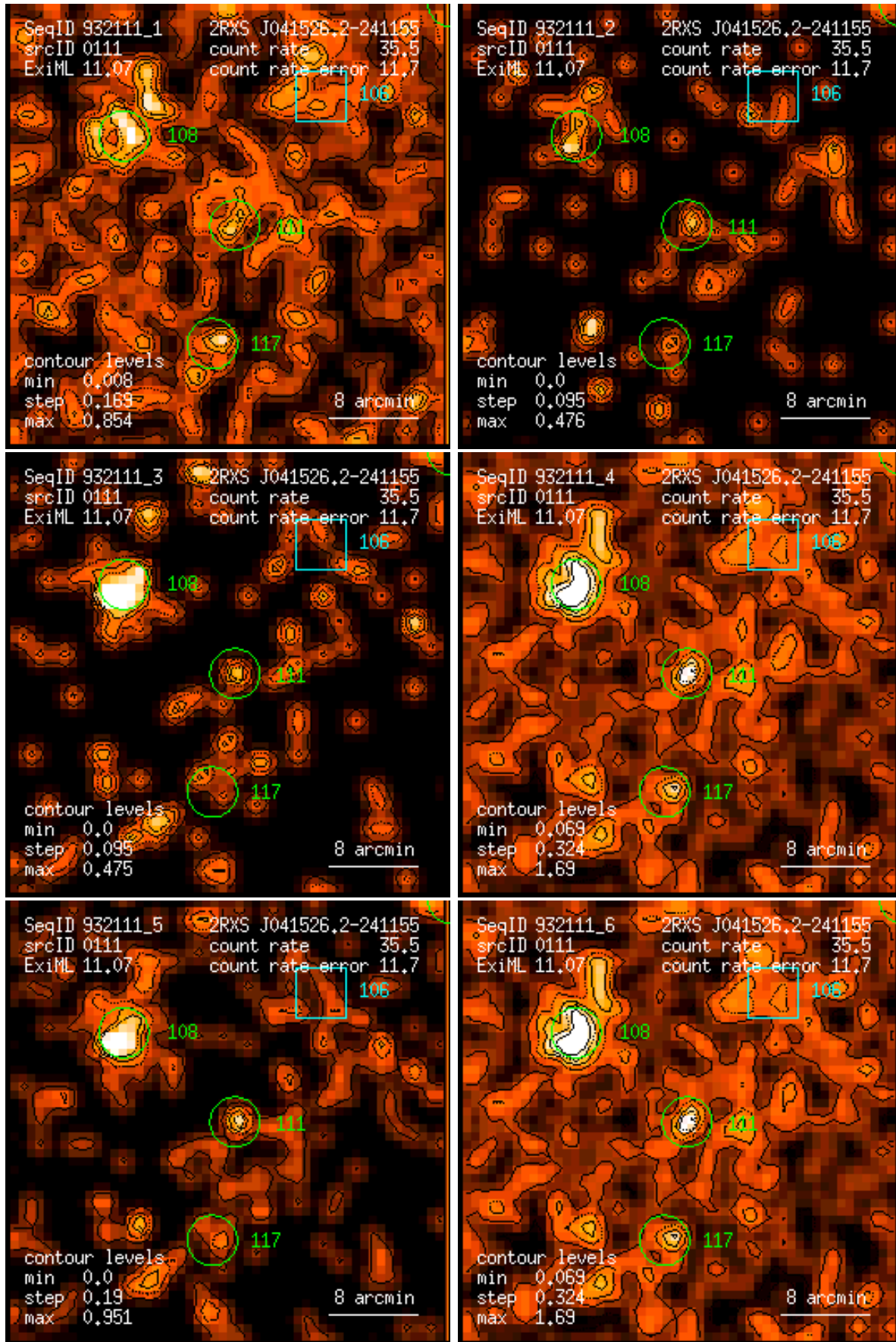
Figure 111: RASS 932111: detection 0111: band rate images, Gaussian filter: (1) PSPC channels 11 – 41, (2) 52 – 90, (3) 91 – 201, (4) 11 – 235, (5) 52 – 201, (6) 11 – 201. Broad band rates in counts/ks. Band rate contour levels in counts/ks/arcmin 2 .
