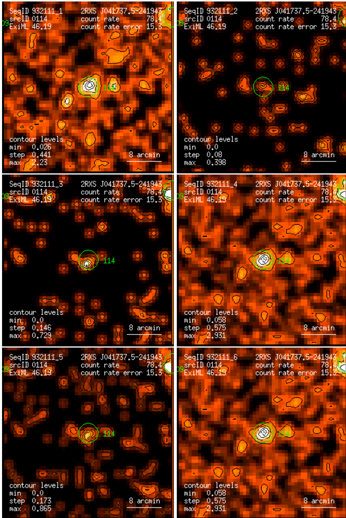
Figure 114: RASS 932111: detection 0114: band rate images, Gaussian filter: (1) PSPC channels 11 – 41, (2) 52 – 90, (3) 91 – 201, (4) 11 – 235, (5) 52 – 201, (6) 11 – 201. Broad band rates in counts/ks. Band rate contour levels in counts/ks/arcmin 2 .
