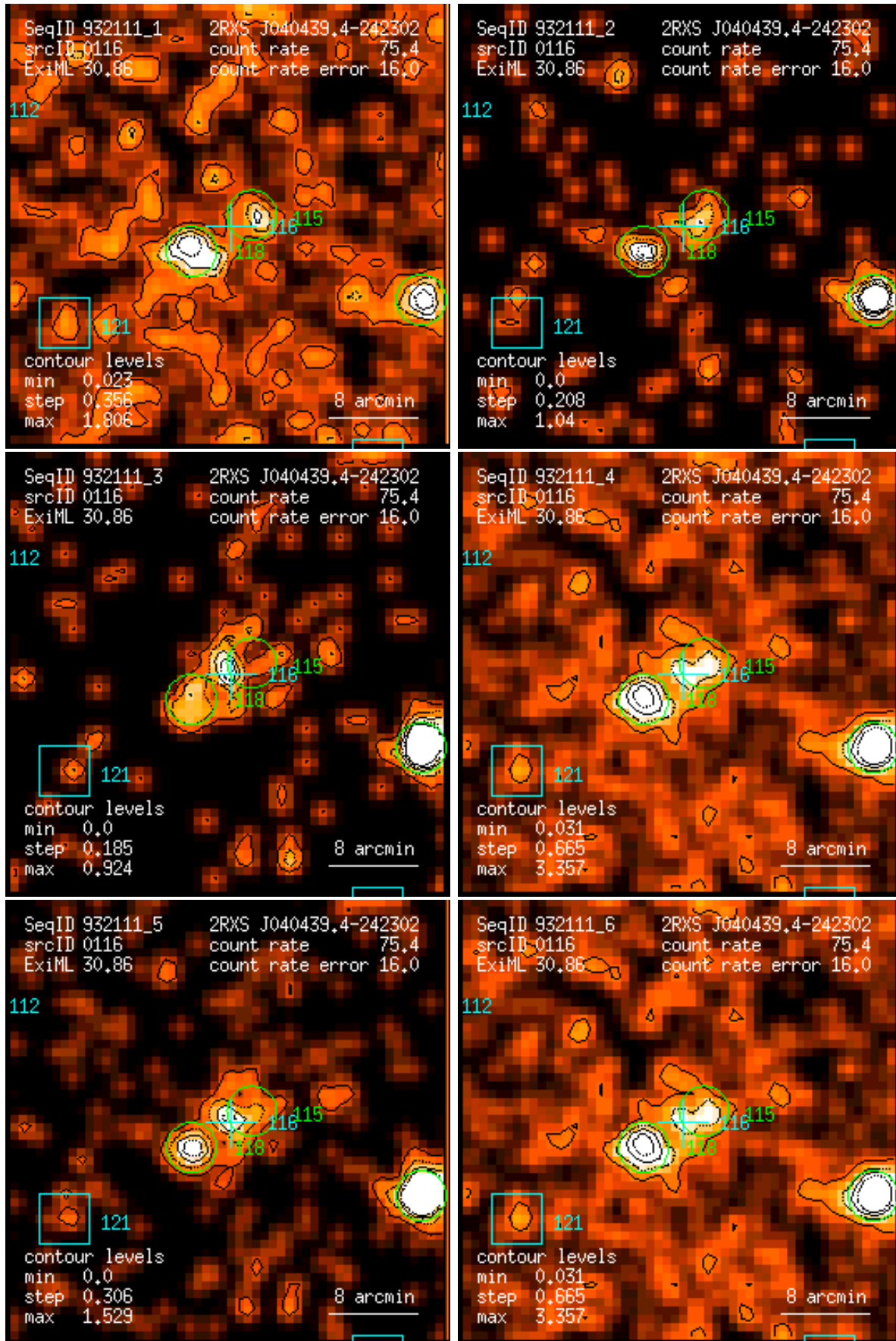
Figure 116: RASS 932111: detection 0116: band rate images, Gaussian filter: (1) PSPC channels 11 – 41, (2) 52 – 90, (3) 91 – 201, (4) 11 – 235, (5) 52 – 201, (6) 11 – 201. Broad band rates in counts/ks. Band rate contour levels in counts/ks/arcmin 2 .
