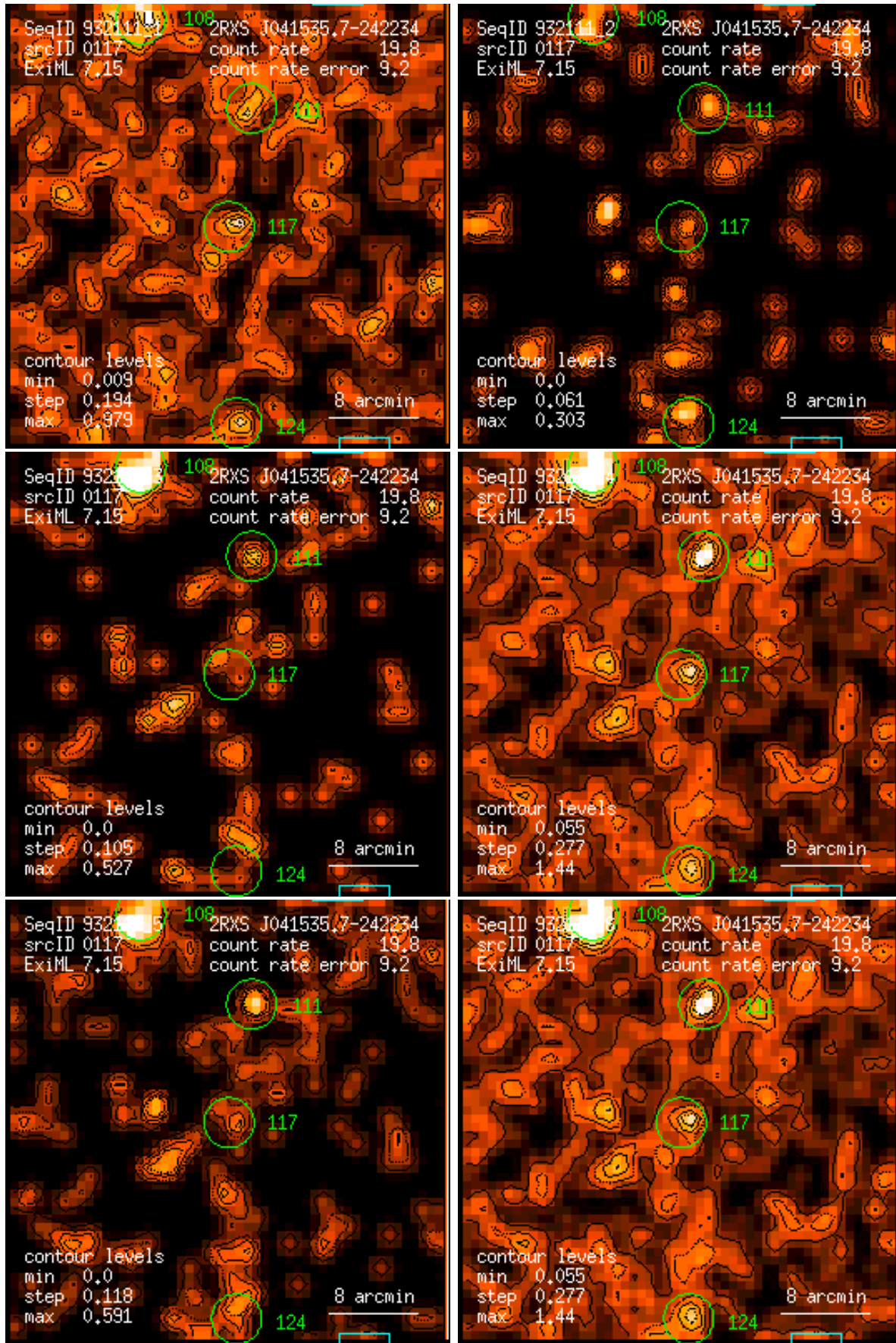
Figure 117: RASS 932111: detection 0117: band rate images, Gaussian filter: (1) PSPC channels 11 – 41, (2) 52 – 90, (3) 91 – 201, (4) 11 – 235, (5) 52 – 201, (6) 11 – 201. Broad band rates in counts/ks. Band rate contour levels in counts/ks/arcmin 2 .
