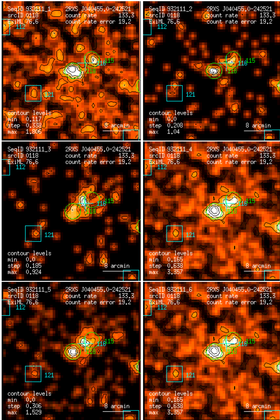
Figure 118: RASS 932111: detection 0118: band rate images, Gaussian filter: (1) PSPC channels 11 – 41, (2) 52 – 90, (3) 91 – 201, (4) 11 – 235, (5) 52 – 201, (6) 11 – 201. Broad band rates in counts/ks. Band rate contour levels in counts/ks/arcmin 2 .
