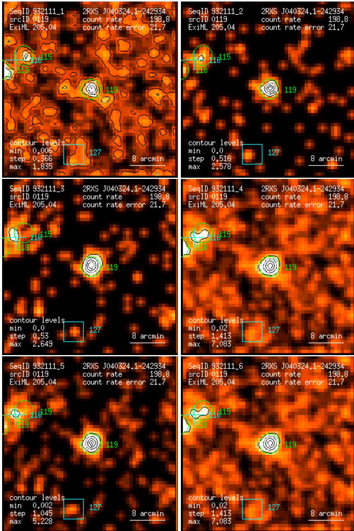
Figure 119: RASS 932111: detection 0119: band rate images, Gaussian filter: (1) PSPC channels 11 – 41, (2) 52 – 90, (3) 91 – 201, (4) 11 – 235, (5) 52 – 201, (6) 11 – 201. Broad band rates in counts/ks. Band rate contour levels in counts/ks/arcmin 2 .
