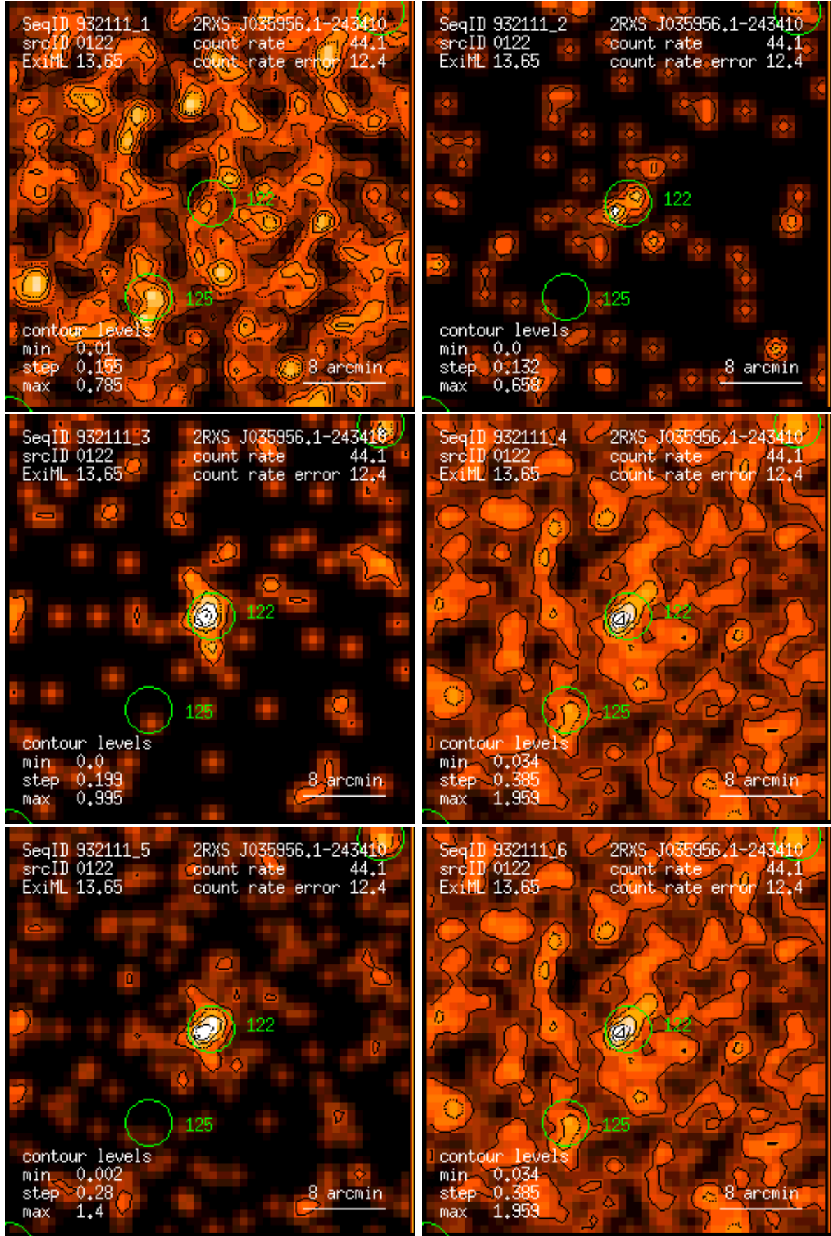
Figure 122: RASS 932111: detection 0122: band rate images, Gaussian filter: (1) PSPC channels 11 – 41, (2) 52 – 90, (3) 91 – 201, (4) 11 – 235, (5) 52 – 201, (6) 11 – 201. Broad band rates in counts/ks. Band rate contour levels in counts/ks/arcmin 2 .
