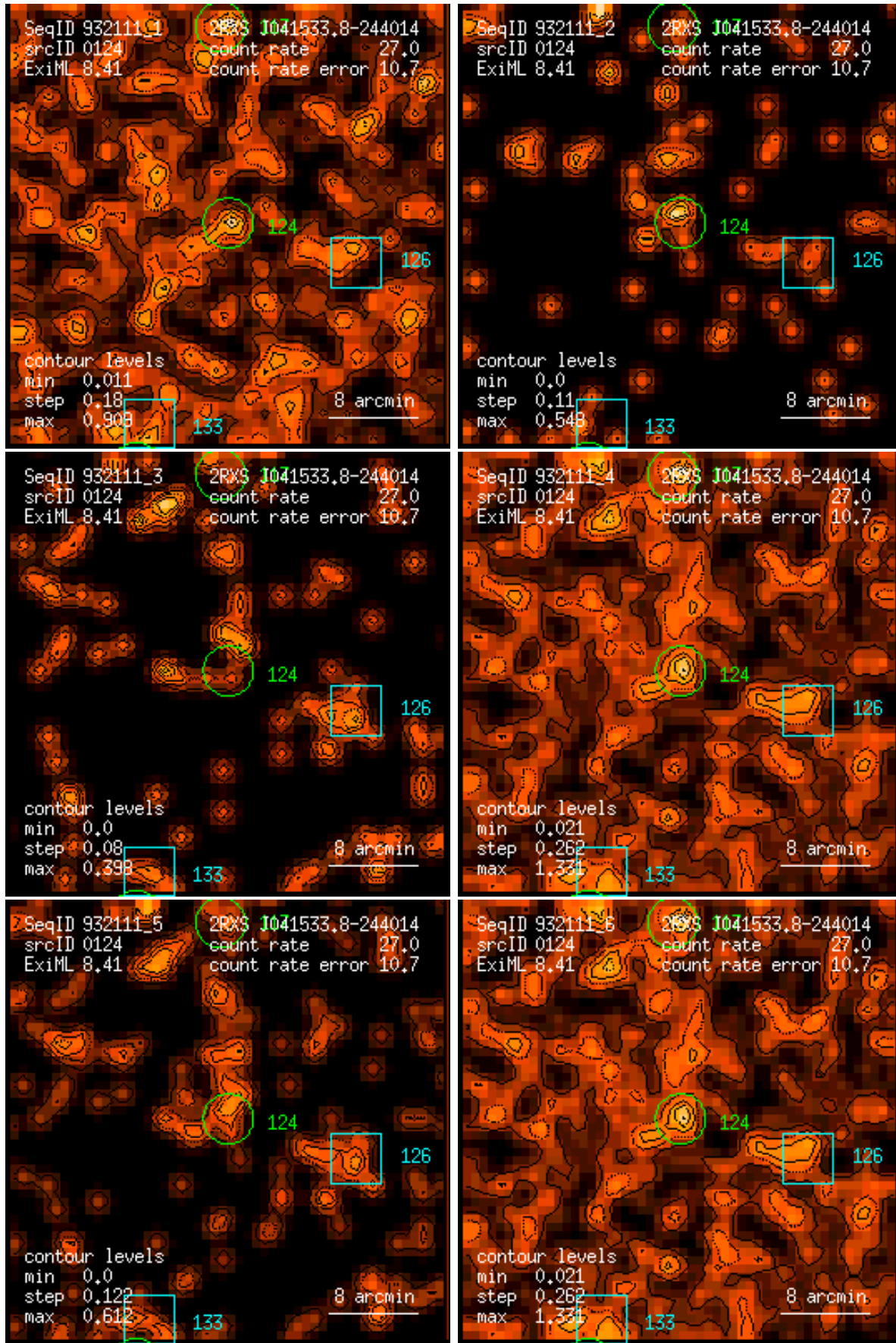
Figure 124: RASS 932111: detection 0124: band rate images, Gaussian filter: (1) PSPC channels 11 – 41, (2) 52 – 90, (3) 91 – 201, (4) 11 – 235, (5) 52 – 201, (6) 11 – 201. Broad band rates in counts/ks. Band rate contour levels in counts/ks/arcmin 2 .
