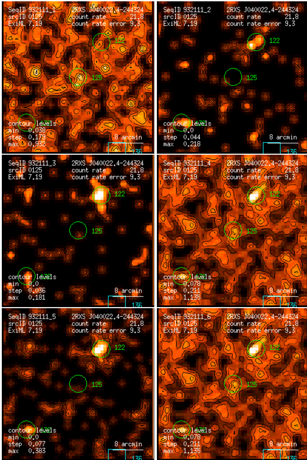
Figure 125: RASS 932111: detection 0125: band rate images, Gaussian filter: (1) PSPC channels 11 – 41, (2) 52 – 90, (3) 91 – 201, (4) 11 – 235, (5) 52 – 201, (6) 11 – 201. Broad band rates in counts/ks. Band rate contour levels in counts/ks/arcmin 2 .
