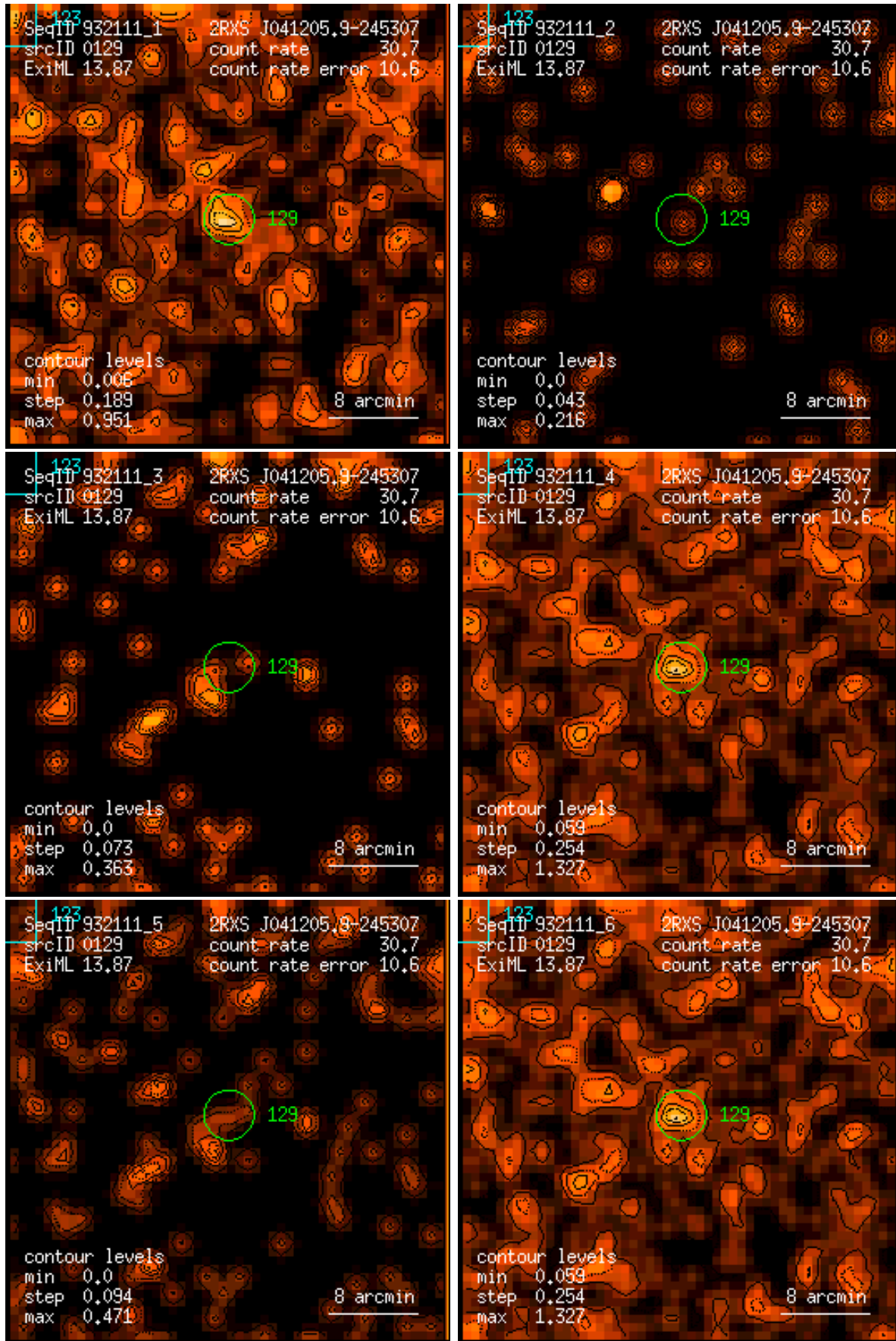
Figure 129: RASS 932111: detection 0129: band rate images, Gaussian filter: (1) PSPC channels 11 – 41, (2) 52 – 90, (3) 91 – 201, (4) 11 – 235, (5) 52 – 201, (6) 11 – 201. Broad band rates in counts/ks. Band rate contour levels in counts/ks/arcmin 2 .
