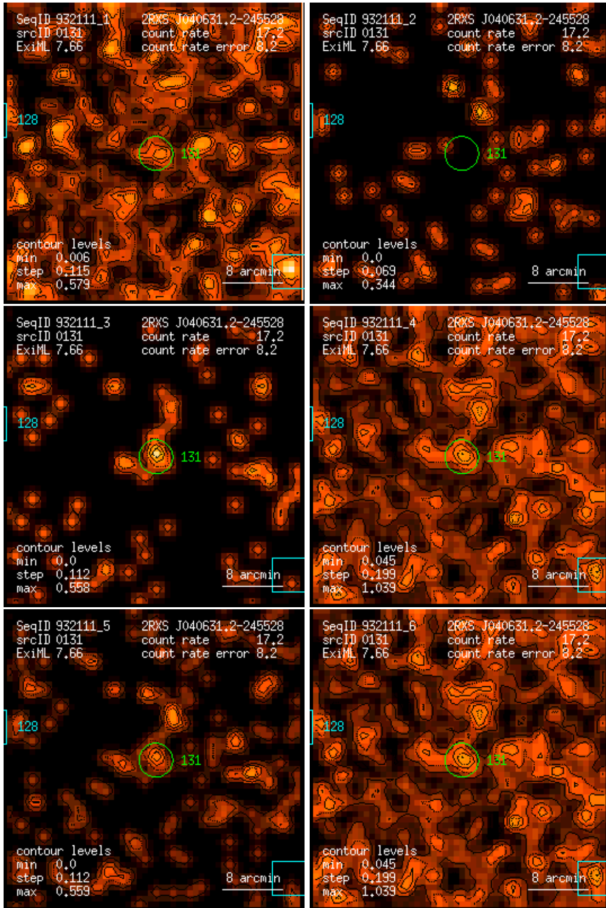
Figure 131: RASS 932111: detection 0131: band rate images, Gaussian filter: (1) PSPC channels 11 – 41, (2) 52 – 90, (3) 91 – 201, (4) 11 – 235, (5) 52 – 201, (6) 11 – 201. Broad band rates in counts/ks. Band rate contour levels in counts/ks/arcmin 2 .
