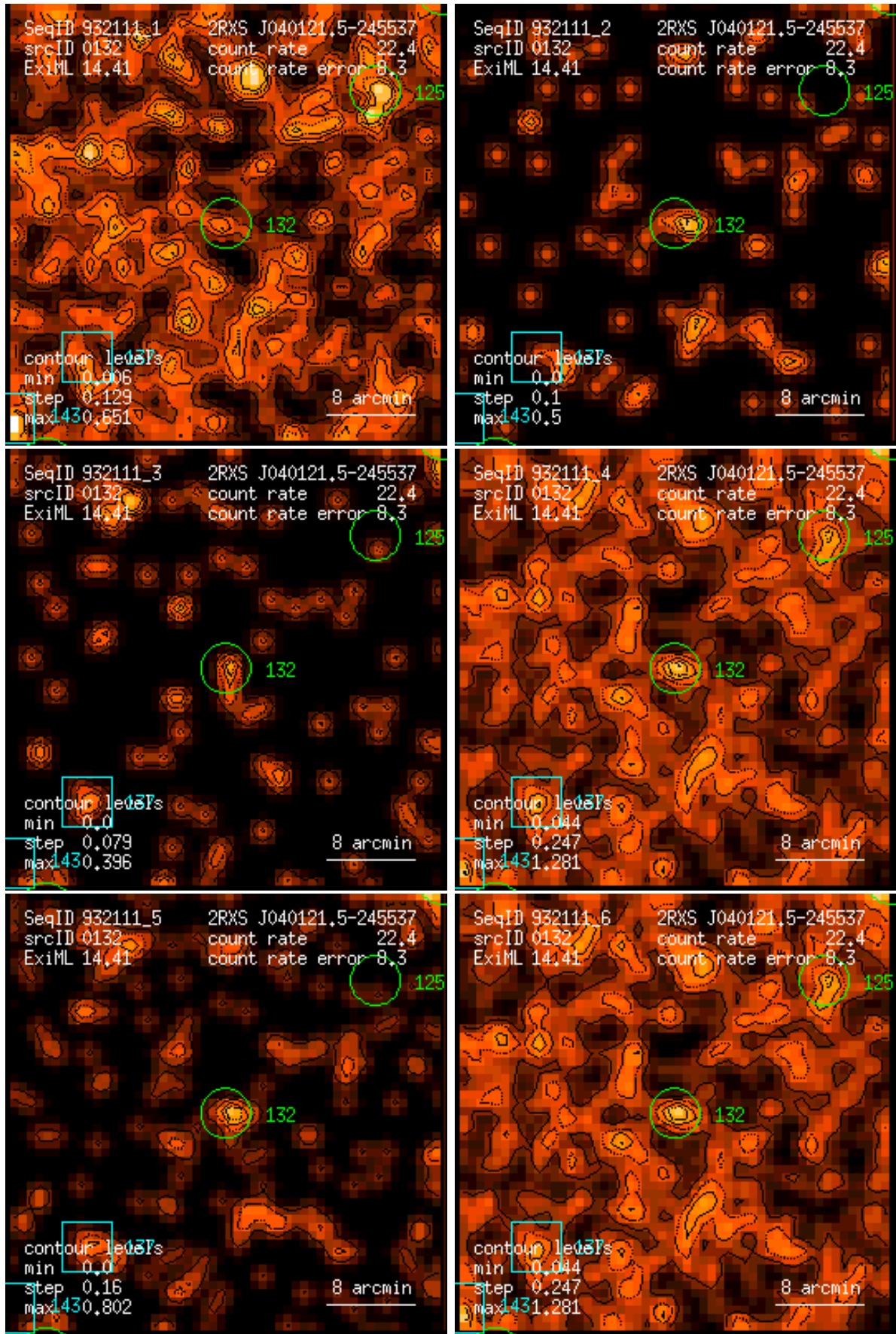
Figure 132: RASS 932111: detection 0132: band rate images, Gaussian filter: (1) PSPC channels 11 – 41, (2) 52 – 90, (3) 91 – 201, (4) 11 – 235, (5) 52 – 201, (6) 11 – 201. Broad band rates in counts/ks. Band rate contour levels in counts/ks/arcmin 2 .
