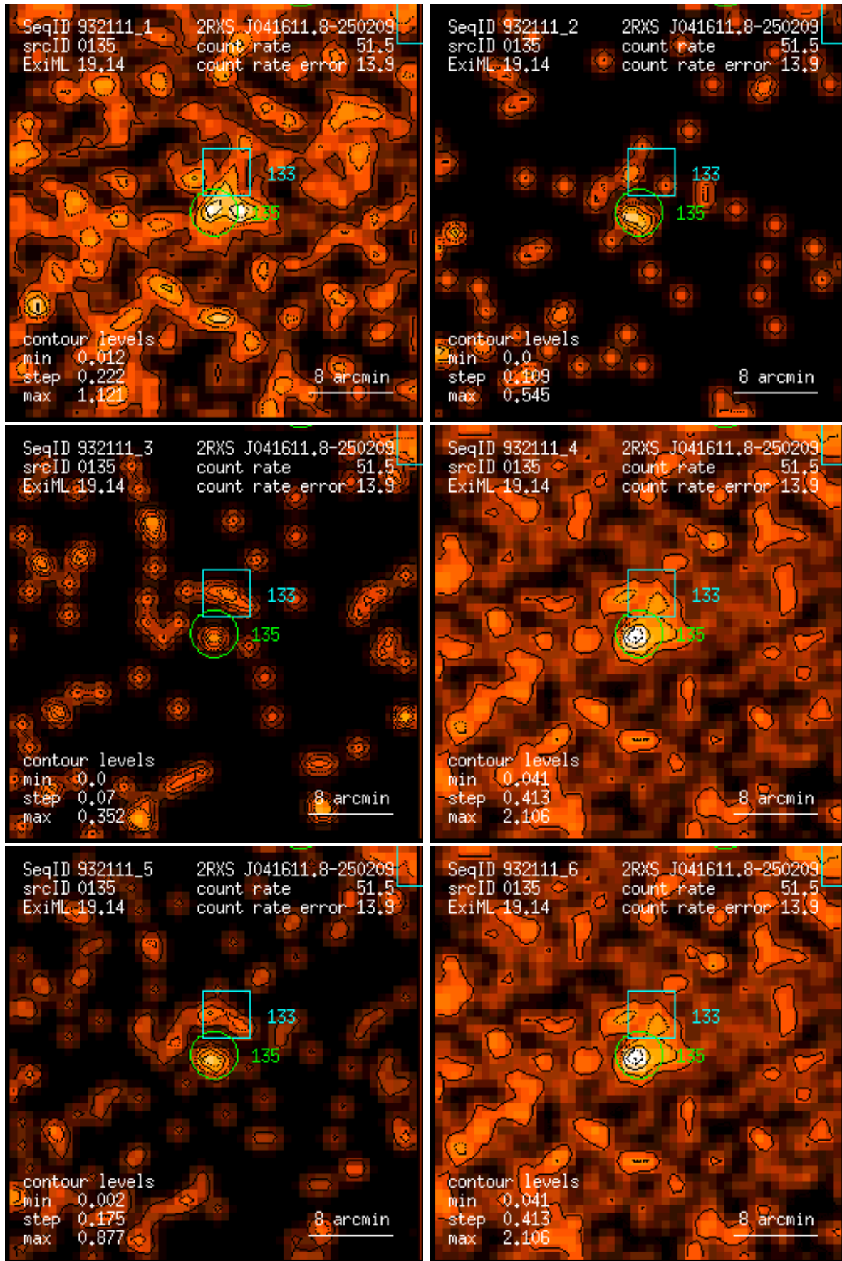
Figure 135: RASS 932111: detection 0135: band rate images, Gaussian filter: (1) PSPC channels 11 – 41, (2) 52 – 90, (3) 91 – 201, (4) 11 – 235, (5) 52 – 201, (6) 11 – 201. Broad band rates in counts/ks. Band rate contour levels in counts/ks/arcmin 2 .
