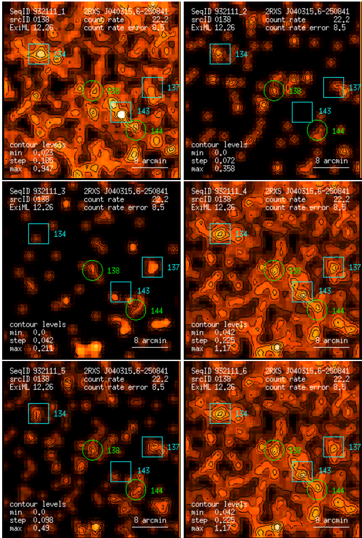
Figure 138: RASS 932111: detection 0138: band rate images, Gaussian filter: (1) PSPC channels 11 – 41, (2) 52 – 90, (3) 91 – 201, (4) 11 – 235, (5) 52 – 201, (6) 11 – 201. Broad band rates in counts/ks. Band rate contour levels in counts/ks/arcmin 2 .
