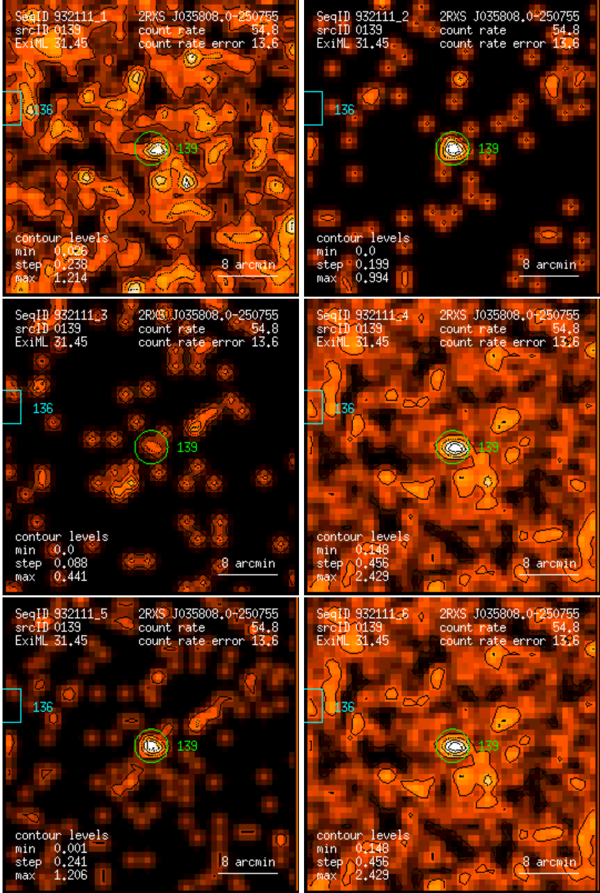
Figure 139: RASS 932111: detection 0139: band rate images, Gaussian filter: (1) PSPC channels 11 – 41, (2) 52 – 90, (3) 91 – 201, (4) 11 – 235, (5) 52 – 201, (6) 11 – 201. Broad band rates in counts/ks. Band rate contour levels in counts/ks/arcmin 2 .
