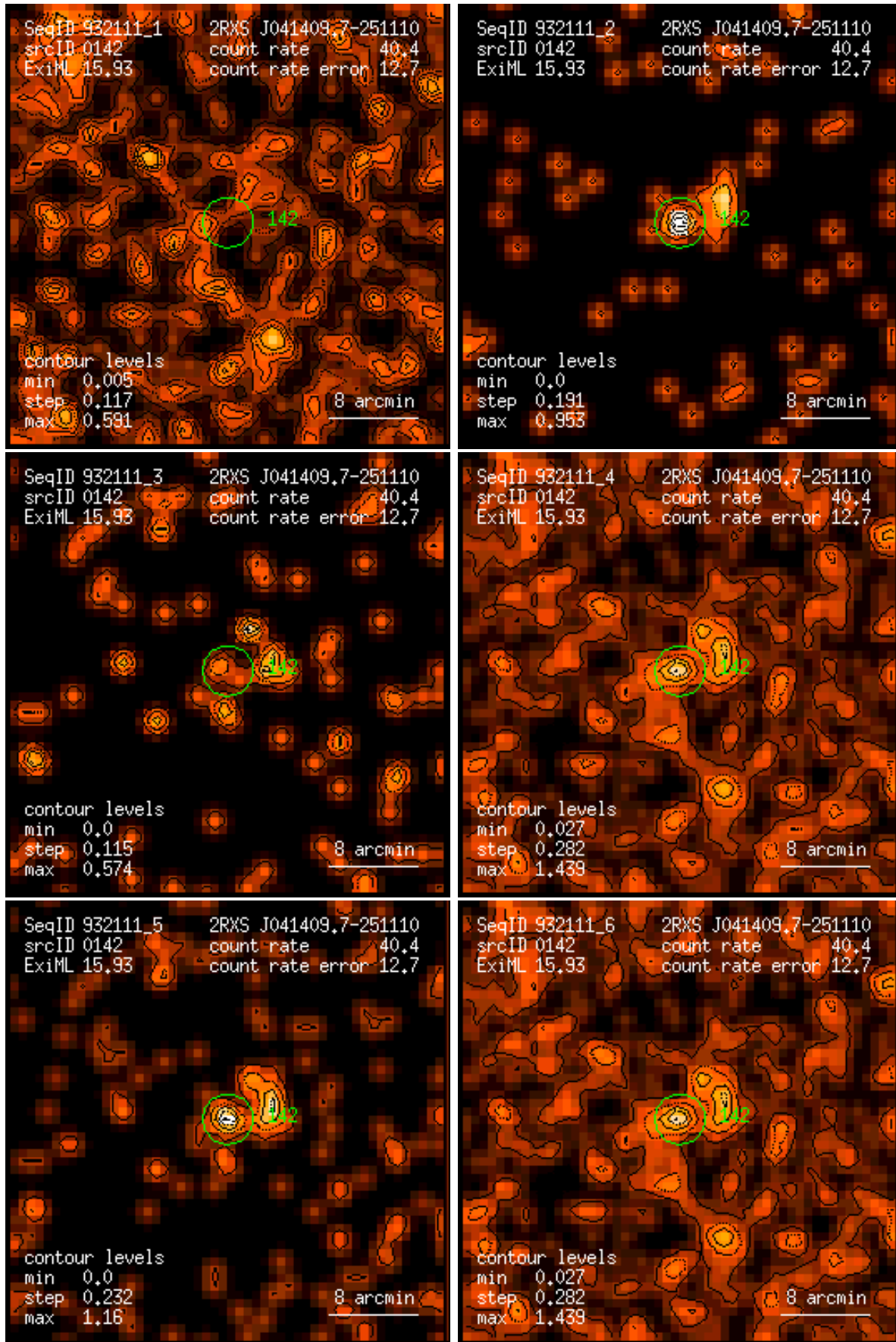
Figure 142: RASS 932111: detection 0142: band rate images, Gaussian filter: (1) PSPC channels 11 – 41, (2) 52 – 90, (3) 91 – 201, (4) 11 – 235, (5) 52 – 201, (6) 11 – 201. Broad band rates in counts/ks. Band rate contour levels in counts/ks/arcmin 2 .
