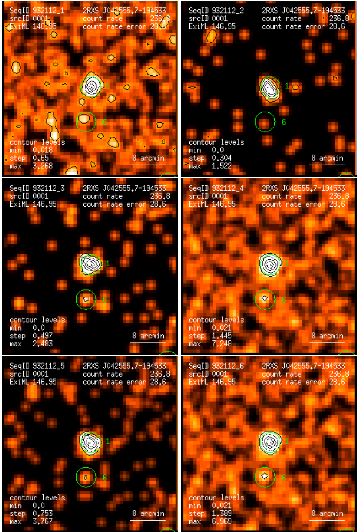
Figure 1: RASS 932112: detection 0001: band rate images, Gaussian filter: (1) PSPC channels 11 – 41, (2) 52 – 90, (3) 91 – 201, (4) 11 – 235, (5) 52 – 201, (6) 11 – 201. Broad band rates in counts/ks. Band rate contour levels in counts/ks/arcmin 2 .
