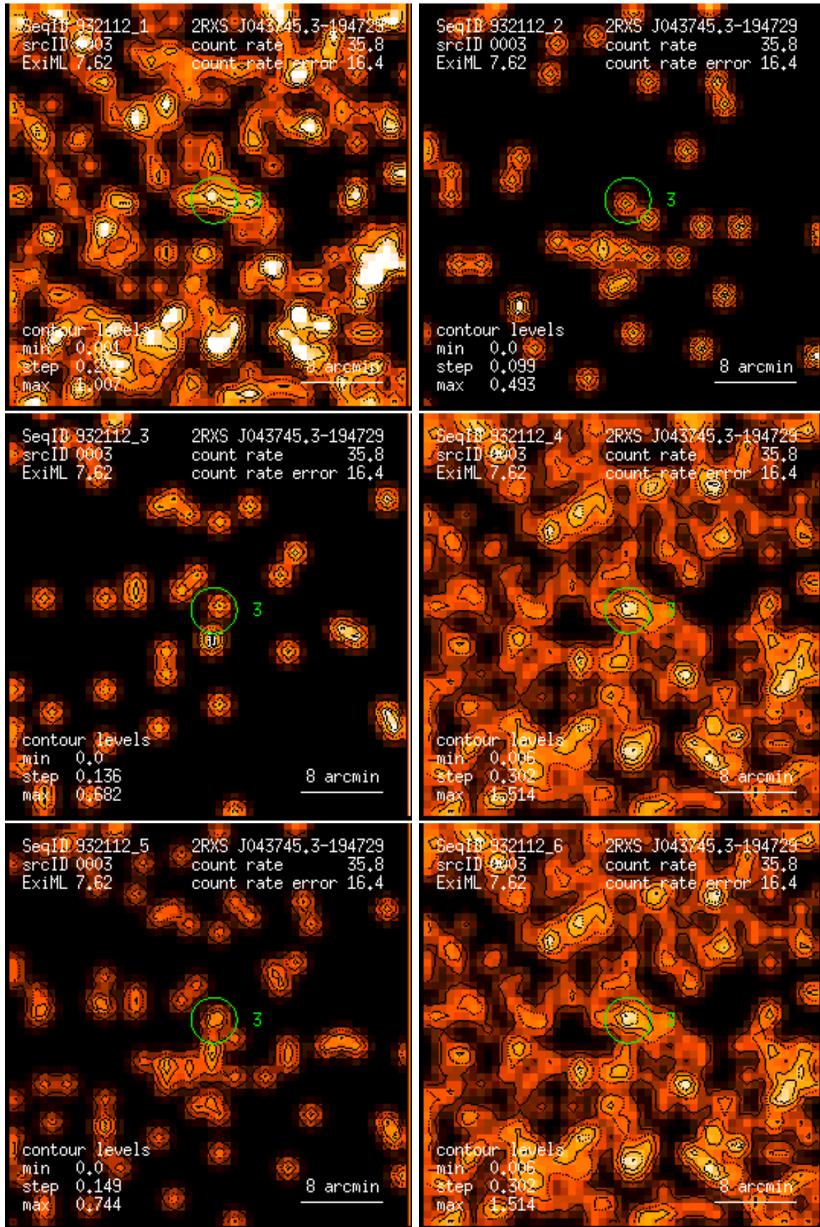
Figure 3: RASS 932112: detection 0003: band rate images, Gaussian filter: (1) PSPC channels 11 – 41, (2) 52 – 90, (3) 91 – 201, (4) 11 – 235, (5) 52 – 201, (6) 11 – 201. Broad band rates in counts/ks. Band rate contour levels in counts/ks/arcmin 2 .
