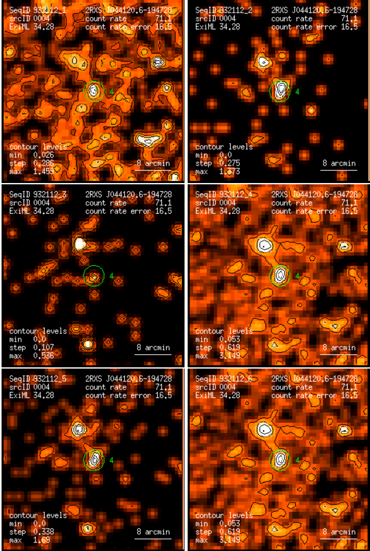
Figure 4: RASS 932112: detection 0004: band rate images, Gaussian filter: (1) PSPC channels 11 – 41, (2) 52 – 90, (3) 91 – 201, (4) 11 – 235, (5) 52 – 201, (6) 11 – 201. Broad band rates in counts/ks. Band rate contour levels in counts/ks/arcmin 2 .
