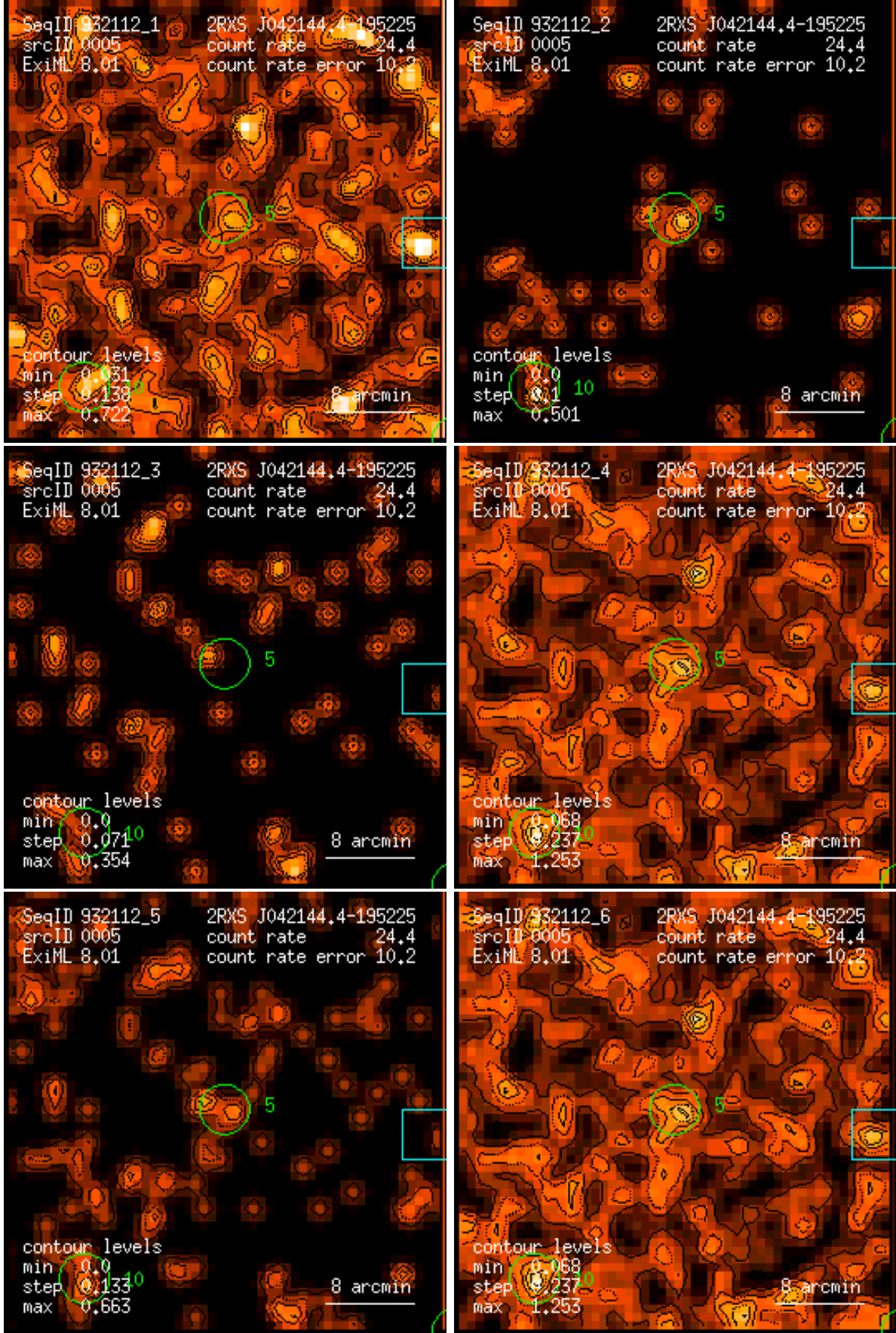
Figure 5: RASS 932112: detection 0005: band rate images, Gaussian filter: (1) PSPC channels 11 – 41, (2) 52 – 90, (3) 91 – 201, (4) 11 – 235, (5) 52 – 201, (6) 11 – 201. Broad band rates in counts/ks. Band rate contour levels in counts/ks/arcmin 2 .
