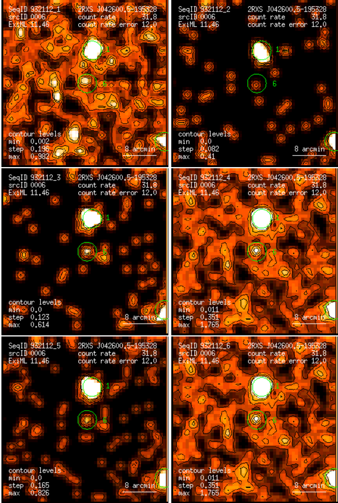
Figure 6: RASS 932112: detection 0006: band rate images, Gaussian filter: (1) PSPC channels 11 – 41, (2) 52 – 90, (3) 91 – 201, (4) 11 – 235, (5) 52 – 201, (6) 11 – 201. Broad band rates in counts/ks. Band rate contour levels in counts/ks/arcmin 2 .
