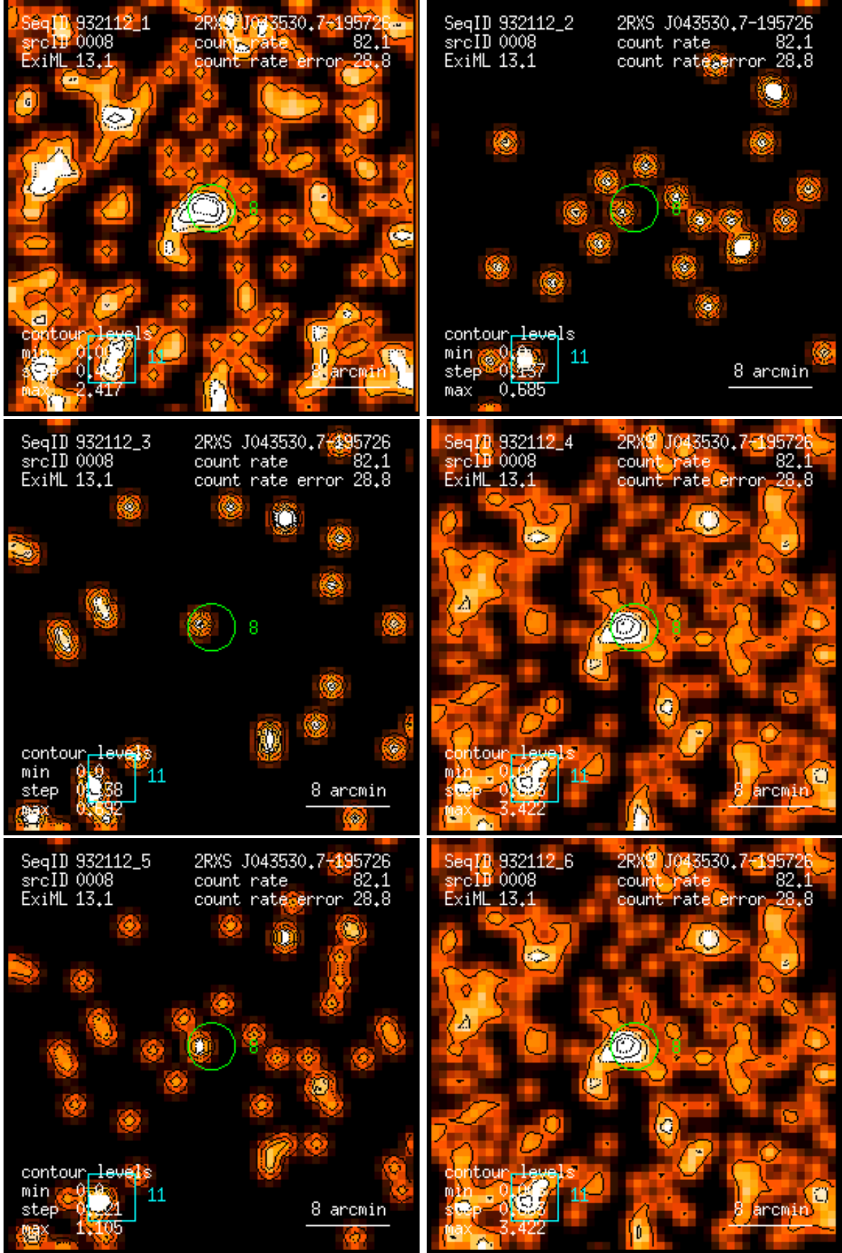
Figure 8: RASS 932112: detection 0008: band rate images, Gaussian filter: (1) PSPC channels 11 – 41, (2) 52 – 90, (3) 91 – 201, (4) 11 – 235, (5) 52 – 201, (6) 11 – 201. Broad band rates in counts/ks. Band rate contour levels in counts/ks/arcmin 2 .
