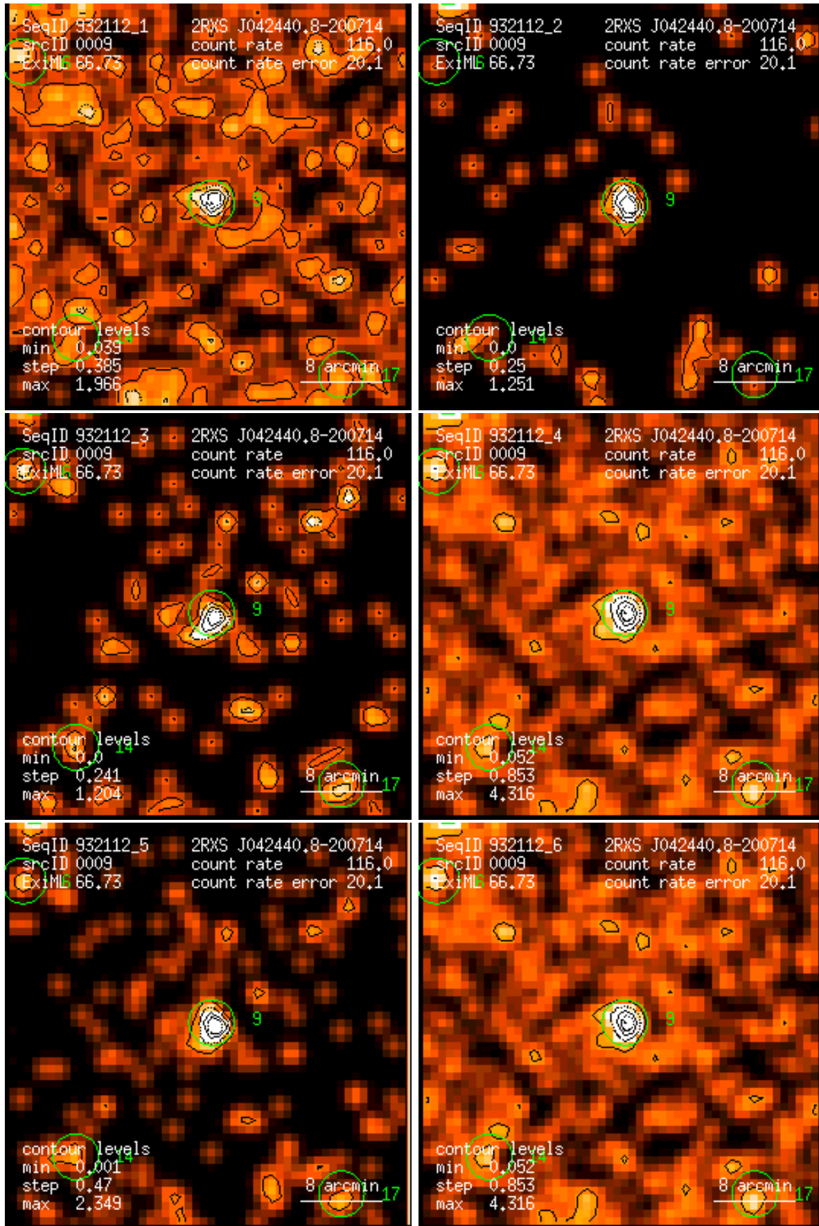
Figure 9: RASS 932112: detection 0009: band rate images, Gaussian filter: (1) PSPC channels 11 – 41, (2) 52 – 90, (3) 91 – 201, (4) 11 – 235, (5) 52 – 201, (6) 11 – 201. Broad band rates in counts/ks. Band rate contour levels in counts/ks/arcmin 2 .
